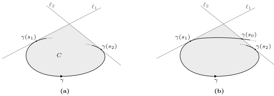
Fig. 1 The curve \gamma in the proof of Lemma 2.7
