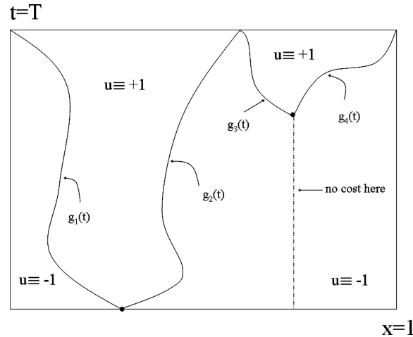
Fig. 3 In the sharp-interface limit, the action is expected to count two costs: the cost of interface nucleation and the cost of interface propagation . See Theorem 1.4
