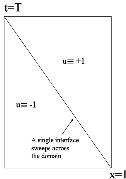
Fig. 1 When the domain is sufficiently small, the sharp-interface action minimizer nucleates a single interface at time t = 0 and propagates it across the domain at a constant velocity.
