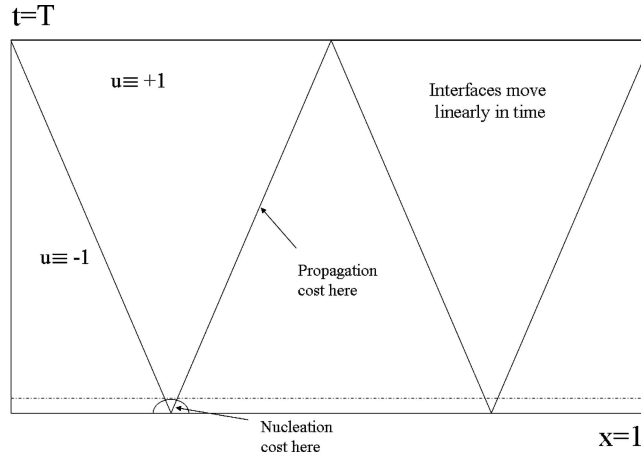
Fig. 2 Given a shorter time to switch or a bigger domain, the action minimizer generates more than one interface in order to reduce the “propagation cost.” Heuristics suggest that the optimal pathway generates all interfaces immediately, and propagates each with the same, constant speed. Theorem 1.3 proves that such behavior does indeed lead to the optimal action in the limit \varepsilon \rightarrow 0 . Theorem 1.4 proves that under the assumption of single-multiplicity interfaces, any optimal path must behave in this way.
