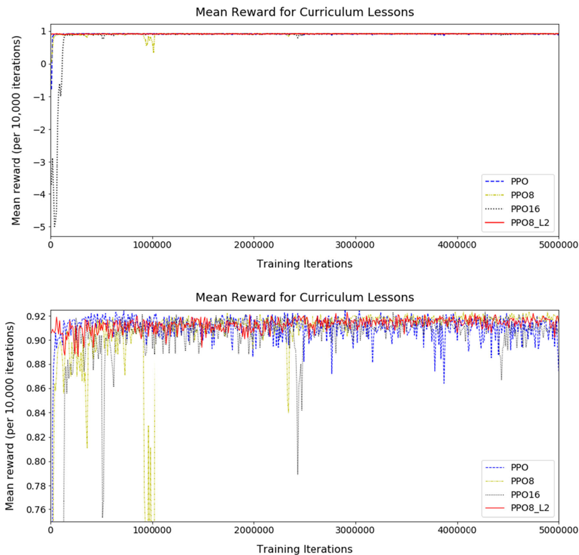
Fig. 7 Line plots of mean reward on the y-axis (averaged over each 10,000 iterations) with iteration number on the x-axis for PPO, PPO 8 and PPO 16 on the first lesson of the curriculum (16 × 16 grid with 1
