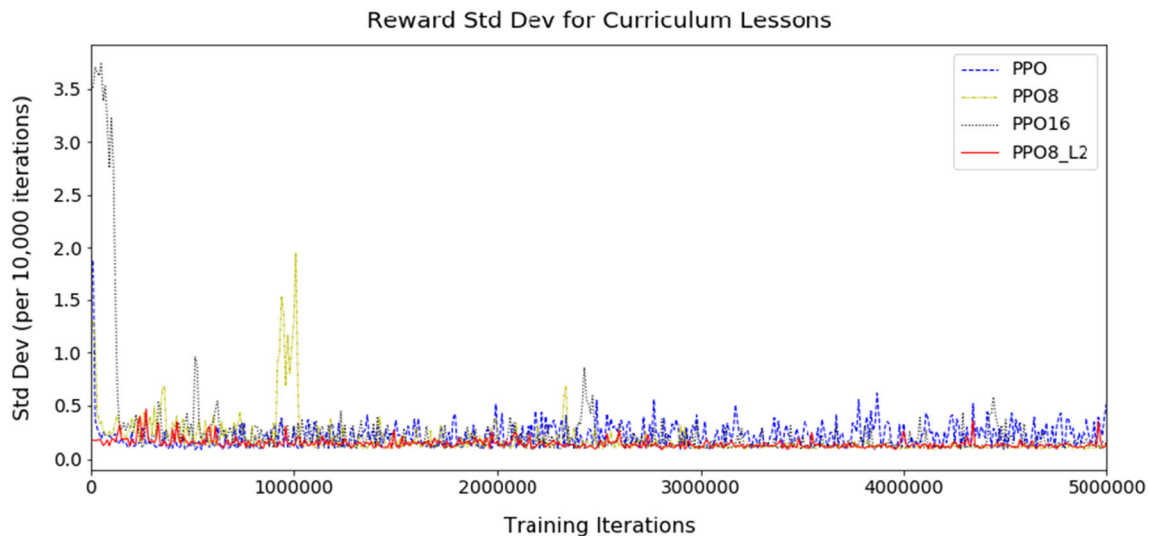
Fig. 8 Line plot of reward standard deviation on the y-axis (over each 10,000 iterations) with iteration number on the x-axis for PPO, PPO 8 and PPO 16 on the first lesson of the curriculum (16 × 16 grid with 1
