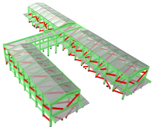
Fig. 16 Structural model
