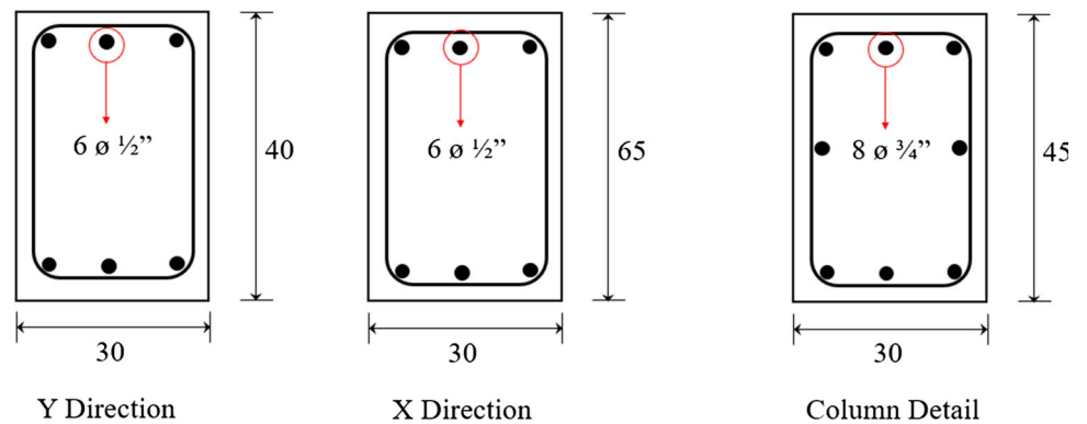
Beam Detail
