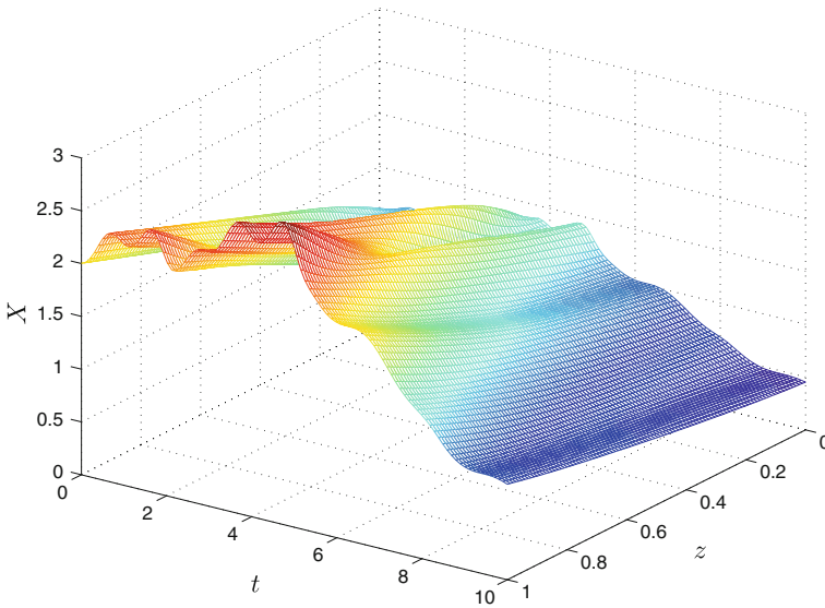
Fig. 1 Solution of (26) for t \in [0, 10] and for z \in [0, 1]
