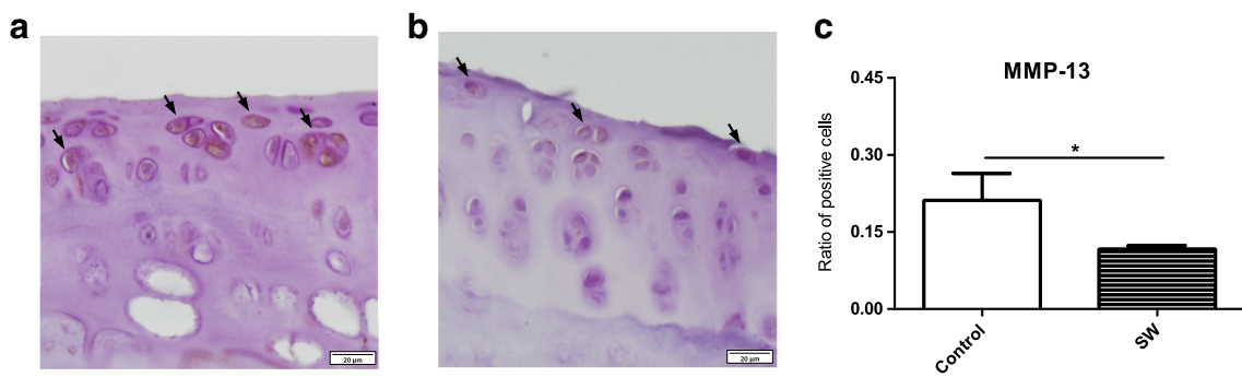
Fig. 5 MMP-13 expression in the articular cartilage. Representative samples of MMP-13 immunohistochemistry in the cartilage from control ( a ) or balneotherapy in sulfurous water group ( b ). Arrows indicate positive cells for immunostaining. c Quantitative analysis of MMP-13-
