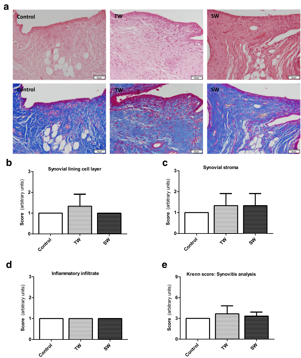
Fig. 4 Histological analysis of synovial tissue. Pathological responses in the synovial tissue were evaluated by semi-quantitative Krenn score as previously indicated in the “Material and methods” section. a Representative images of synovial sections stained with hematoxylin and eosin (above) and Masson’s trichrome (below) from each group of study. Analysis of semi-quantitative score of the following pathological alterations in the synovial tissue: Number of lining cell layers ( b ), proliferation of the subintima tissue ( c ), and infiltration of inflammatory cells ( d ). e The sum of the pathological changes in the tissue is shown. Values are mean ± SEM ( n = 3 independent animals for each condition). No significant differences were found. Control, non-treated; TW, balneotherapy in tap water; SW, balneotherapy in sulfurous water
