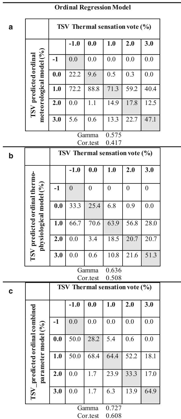
Fig. 4 Cross-tabulation diagram of actual TSV by a ordinal meteorological model, b ordinal thermo-physiological model and c ordinal combined parameter model
