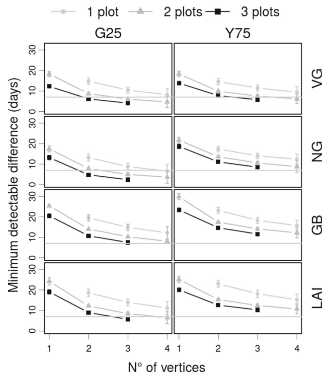
Fig. 5 Minimum detectable difference ( d_{p=0.05} , expressed in days) as a function of number of plots and vertices for phase G25 (left column) and Y75 (right column) of all investigated indices from the sample removal analysis. For reference, a horizontal grey line at 7 days (1 week) is shown. VG visual greening, NG nadiral greening, GB green biomass, LAI leaf area index
