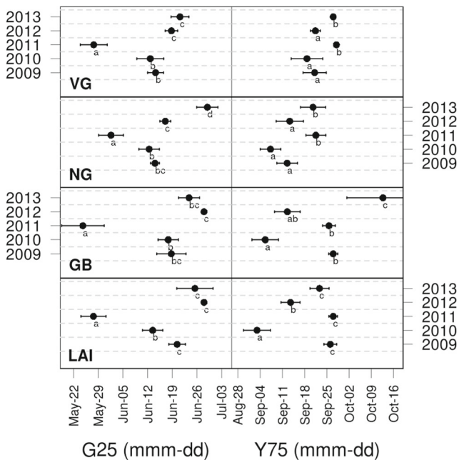
Fig. 3 Mean date of occurrence of phases G25 and Y75 extracted from percentiles on the spline fitting for all indices in 5 years. Error bars represent \pm 2se of the mean. Different letters indicate significant difference ( p < 0.05 ) between the means (Tukey HSD). VG visual greening, NG nadiral greening, GB green biomass, LAI leaf area index
