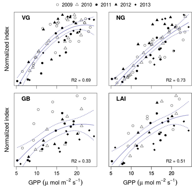
Fig. 4 Scatterplot between seasonal trajectories of the investigated indices and gross primary production (GPP). GPP data represent the mean values for 7-day windows including only fluxes measured during periods with incident photosynthetic photon flux density (PPFD) > 1400 \mu mol m^{-2} s^{-1} . Weekly time windows are centred on the day samples for indices were collected (Flanagan et al. 2002). The coefficient of determination ( r^2 ) of a quadratic fit and its standard error envelope are shown. VG visual greening, NG nadiral greening, GB green biomass, LAI leaf area index
