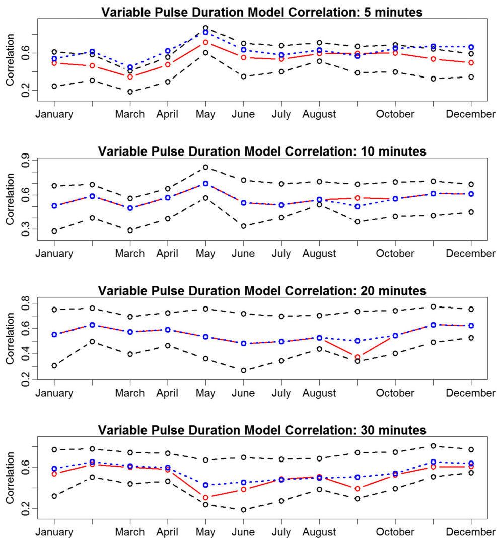
Fig. 5 Observed (red) and fitted (blue) values of the autocorrelation of the aggregated rainfall at h = 1/12, 1/6, 1/3, 1/2 h for the exponential initial pulse depth model with variable pulse duration d , along with simulation bands (black) from 1000 simulations
