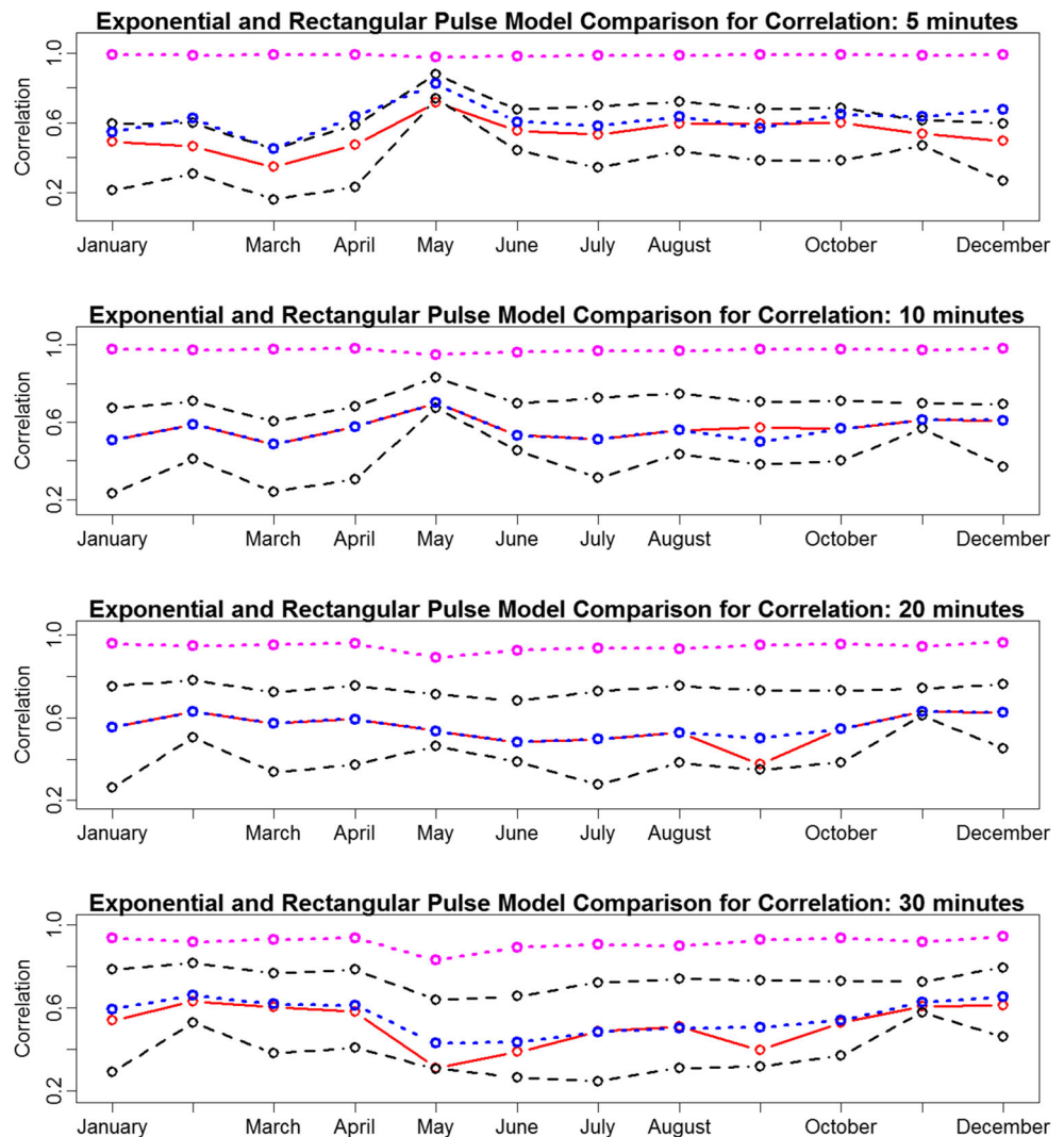
Fig. 12 Observed (red) and fitted (blue) values of the autocorrelation of the aggregated rainfall at h = 1/12, 1/6, 1/3, 1/2 h for the exponential initial pulse depth model, along with simulation bands (black) from 1000 simulations. The pink line is for the rectangular pulse model described in Sect. 5
