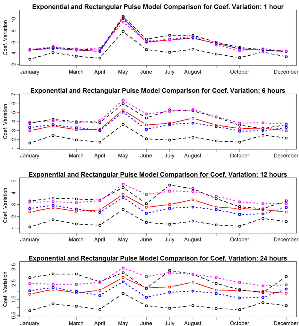
Fig. 14 Observed (red) and fitted (blue) values of the coefficient of variation of the aggregated rainfall at h = 1, 6, 12, 24 h for the exponential initial pulse depth model, along with simulation bands (black) from 1000 simulations. The pink line is for the rectangular pulse model described in Sect. 5
