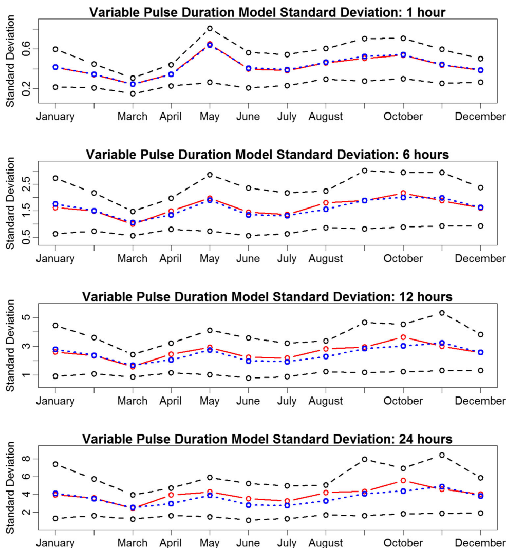
Fig. 4 Observed (red) and fitted (blue) values of the standard deviation of the aggregated rainfall at h = 1, 6, 12, 24 h for the exponential initial pulse depth model with variable pulse duration d , along with simulation bands (black) from 1000 simulations
