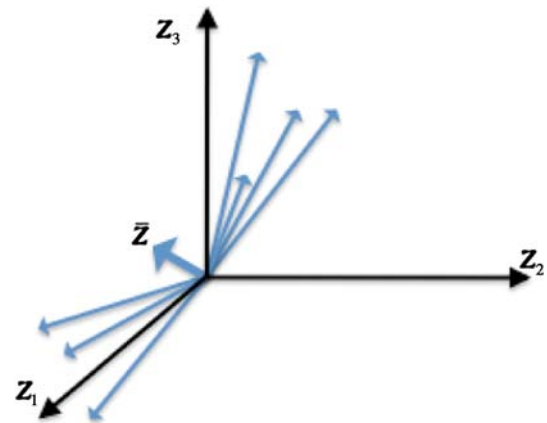
Fig. 2 Example of Result 2. Weak correspondence allows MSE(Z^{(\min)}) \geq MSE(\bar{Z})
