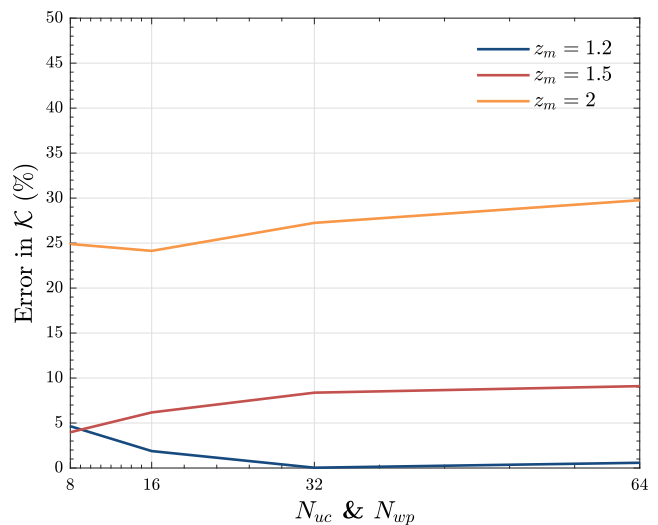
Fig. 14 Global influences of N_{uc} and N_{wp} on strain energy (left) and kinetic energy (right) for various impedance contrast factors. Error estimations in macroscopic displacements are computed based on the DNS solutions
