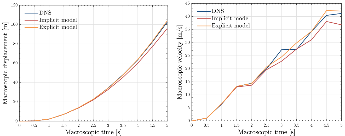
Fig. 11 Comparisons of implicit and explicit model with the reference solution obtained by the DNS regarding macroscopic displacement-time (left) and velocity-time (right) curves at the values of N_{uc} = 8 and N_{wp} = 8
