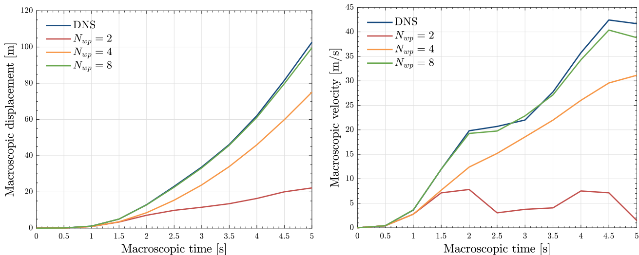
Fig. 9 Macroscopic displacement-time (left) and velocity-time (right) curves at the value of N_{uc} = 8 for various N_{wp} values with the reference solution obtained by the DNS
