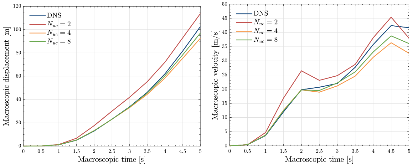
Fig. 7 Macroscopic displacement-time (left) and velocity-time (right) curves for N_{wp} = 8 and various N_{uc} together with the reference solution obtained by the DNS
