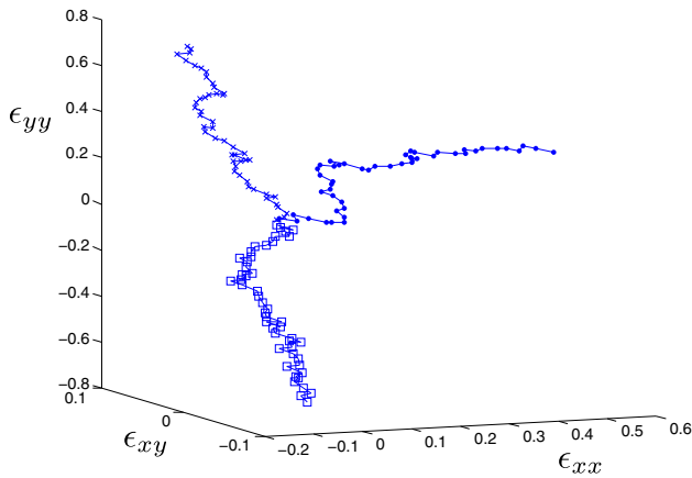
Fig. 7 Example of loading paths obtained using the random procedure
