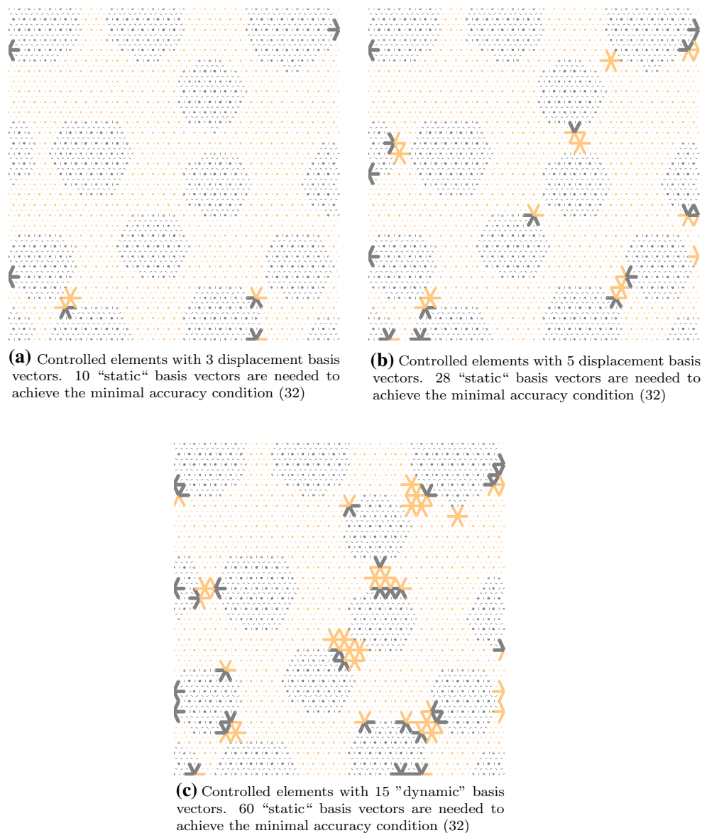
Fig. 9 Controlled elements selected using various basis sizes. The larger the basis, the more controlled elements are needed. The elements tend to gather around the regions where the variation of displacement is the highest, hence where the variation of the internal forces will be high
