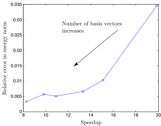
Fig. 12 Evolution of the error with respect to the speedup while increasing the number of basis vectors. For each size of the displacement basis \Phi , the number of vectors in the static basis \Psi is chosen according to the rule defined in Eq. (32)
