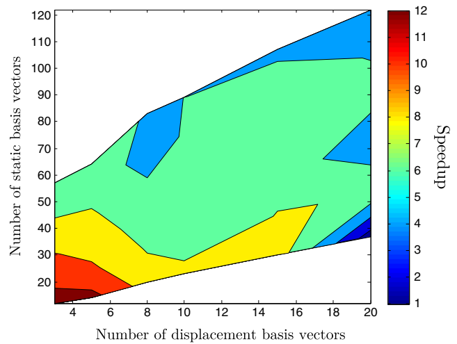
(b) Ratio of time time gained from running the full order model and the reduced model.
