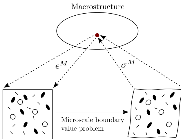
Fig. 1 Semi-concurrent homogenisation procedure. At each macrostructural quadrature point , an RVE boundary value problem can be stated with boundary conditions dictated by the macrostrain at this point . Once the boundary value problem solved, the corresponding macrostress is evaluated as a spatial average of the microstress over the RVE
