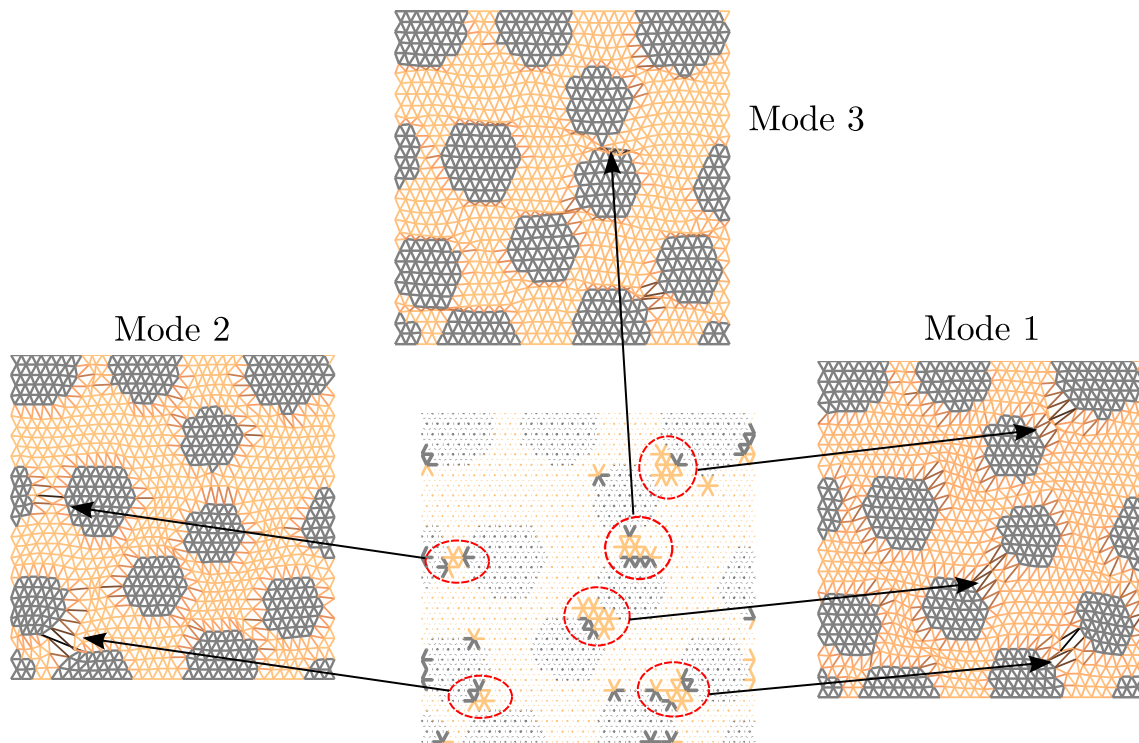
Fig. 10 Regions of interest selected by the system approximation procedure. Those regions (it circled in the figure) are matching the areas of higher displacement found in the POD bases. This is intuitively good, since those elements have to give enough information to be able to
