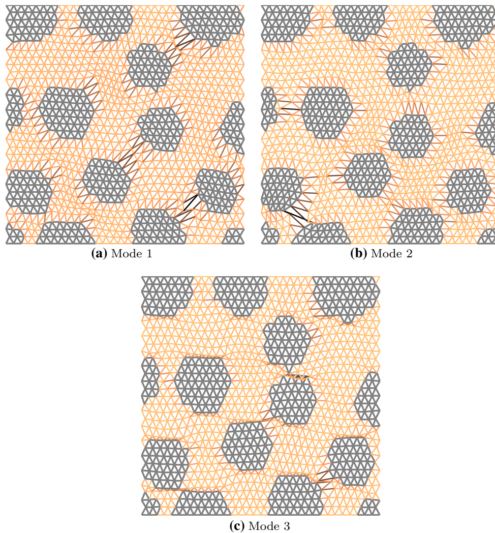
Fig. 8 Vectors associated to the three largest eigenvalues obtained using the snapshot-POD procedure with random snapshot selection. Darker bars indicates larger damage. The damage localises between pairs of inclusions
