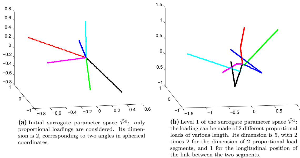
Fig. 13 Examples of loadings paths for levels 0 and 1 of the surrogate parameter spaces
