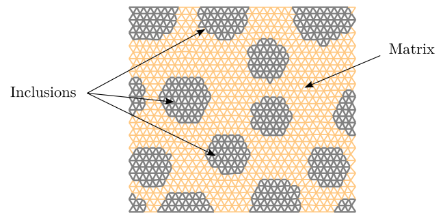
Fig. 2 Lattice model of the computational representative volume element. Beams have different mechanical properties that depend on their location with respect to the distribution of heterogeneities in the computational domain. An arbitrary distribution of inclusions is chosen as a test case for this paper
