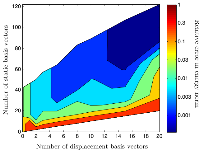
(a) Evolution of the error varying the number of displacement and static basis vectors.
