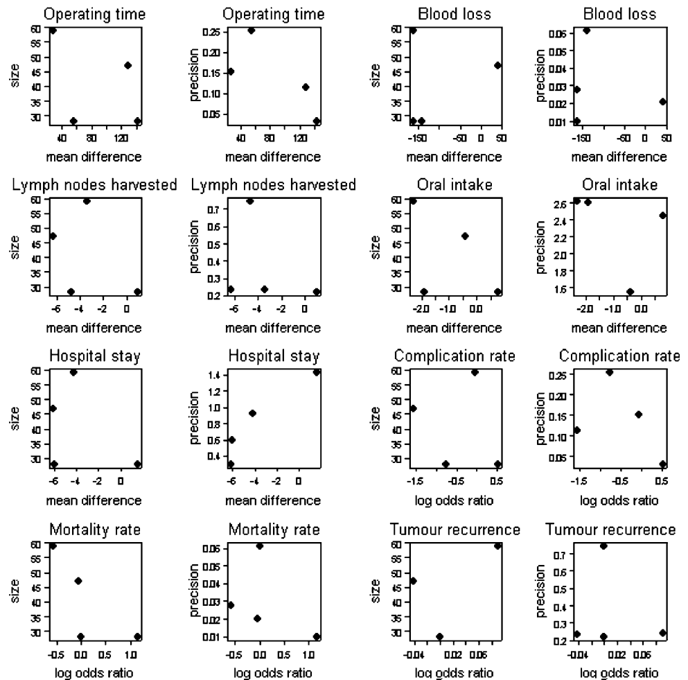
Fig. 1 Funnel plots for every treatment from the studies included in meta-analysis. Precision = 1/standard error
