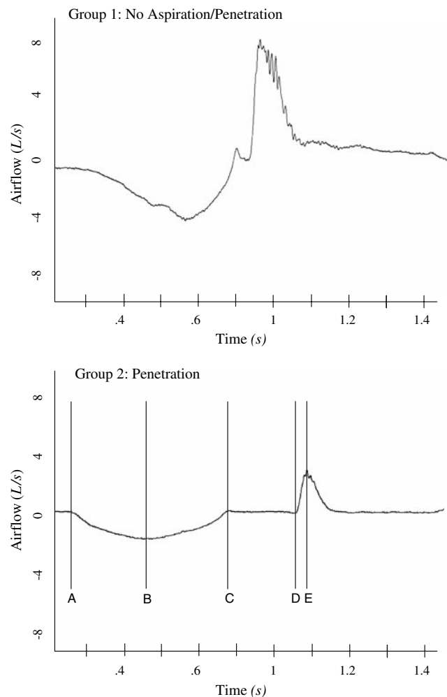
Fig. 1 Examples of airflow waveforms during a voluntary cough task from Group 1 and Group 2. The vertical lines within the Group 2 waveform denote the phases of the cough waveform: A to C, inspiratory phase; C to D, compression phase; D to E, expiratory rise time
