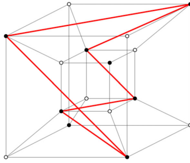
Fig. 1 Longest element representation for the hypertope of type D_4
