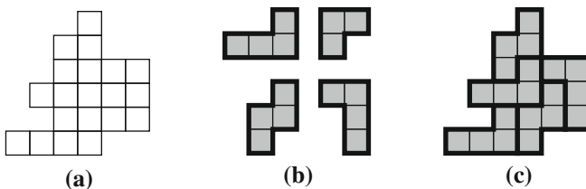
Fig. 1 A Yes-instance (P, S) of the tiling problem consisting of (a) a right-angled polygon P and (b) a set S of polyominoes. (c) Tiling P with polyominoes in S
