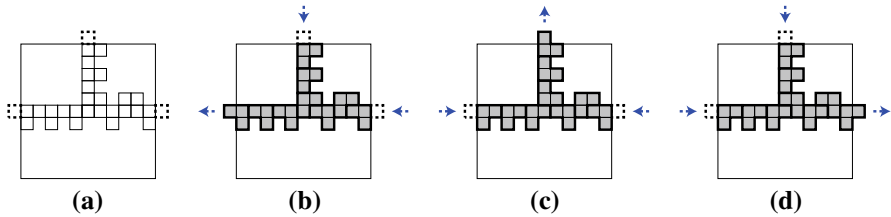
Fig. 11 A negated-clause gadget for L-TILING and LI-TILING, and its three ways of tilings
