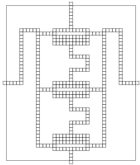
Fig. 18 Gadgets for 2BAR-TILING with S = \{1 \times 2, 3 \times 1\} : (a) line, (b) corner, (c) cross, (d) duplicator, (e) clause and (f) negated-clause gadgets
