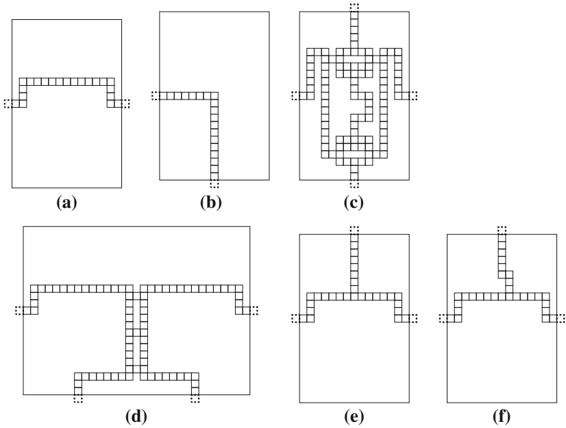
Fig. 18 Gadgets for 2BAR-TILING with S = \{1 \times 2, 3 \times 1\} : (a) line, (b) corner, (c) cross, (d) duplicator, (e) clause and (f) negated-clause gadgets
