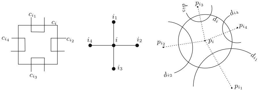
Fig. 27 The pseudocircles c_i, c_{i_1}, c_{i_2}, c_{i_3}, c_{i_4} (left), the corresponding part of the “canonical” embedding of H from Fig. 25 (middle) and the circles d_i, d_{i_1}, d_{i_2}, d_{i_3}, d_{i_4} (right). On the right we have also drawn the relevant edges of the straight-line embedding of H that \mathcal{H}' defines
