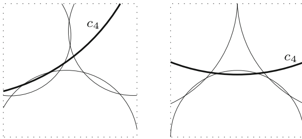
Fig. 16 The arrangements of Fig. 15 are circleable
