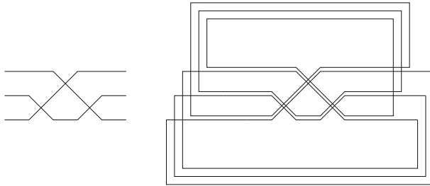
Fig. 34 The construction of the pseudocircle arrangement \mathcal{C} (right) from a simple pseudoline arrangement \mathcal{L} (left)
