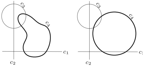
Fig. 7 An arrangement of four pseudocircles in which each pseudocircle intersects exactly two others
