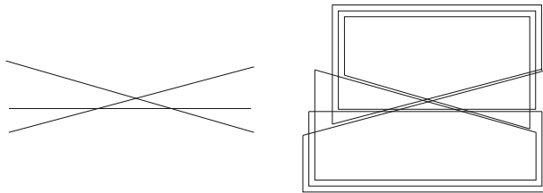
Fig. 35 Repeating the construction when \mathcal{L} is stretchable
