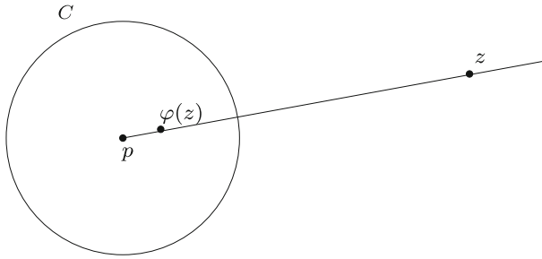
Fig. 3 Inversion in the circle C
