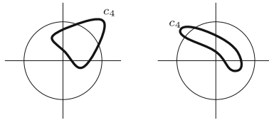
Fig. 13 The situations where (c_1, c_2, c_3) is equivalent to the arrangement in Fig. 6, left, and c_4 does not separate any pair of intersection points
