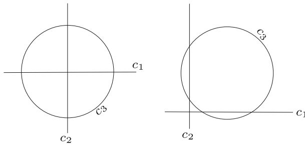
Fig. 6 Two pseudocircle arrangements with n = 3
