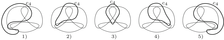
Fig. 15 (c_1, c_2, c_3) is as in Fig. 6, right, c_4 does not separate any pair of intersection points and c_4 intersects some segment exactly once
