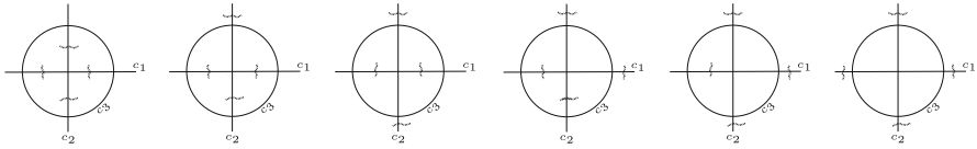
Fig. 11 The situation where (c_1, c_2, c_3) is as in Fig. 6, left, and c_4 surrounds the origin
