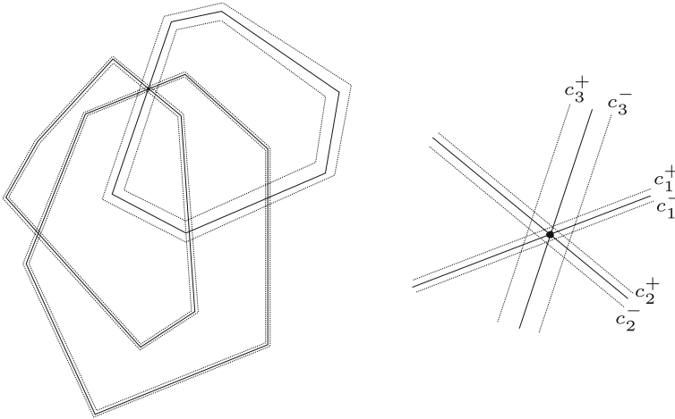
Fig. 33 Replacing each curve of a pencil pseudocircle arrangement by two curves
