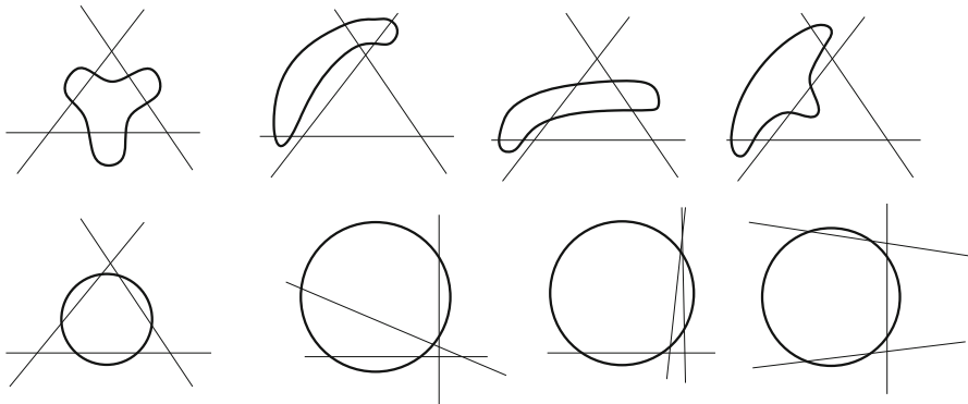
Fig. 24 The curves c_1, c_2, c_3 have exactly one point in common, and c_4 intersects three of them and has none of the three intersection points in its interior
