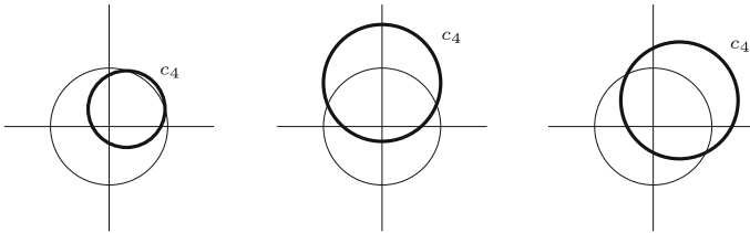
Fig. 12 The arrangements of the first, second and fourth situations in Fig. 11 correspond to circleable arrangements
