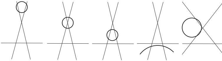
Fig. 22 The curves c_1, c_2, c_3 have exactly one point in common, and c_4 intersects two of them
