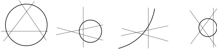
Fig. 23 The curves c_1, c_2, c_3 have exactly one point in common, and c_4 intersects three of them and has at least one of the three intersection points in its interior
