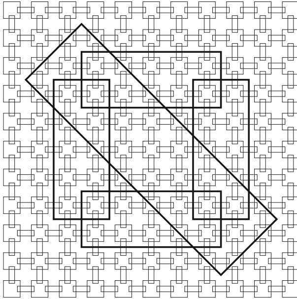
Fig. 2 An arrangement of convex pseudocircles such that no collection of circles defines the same intersection graph
