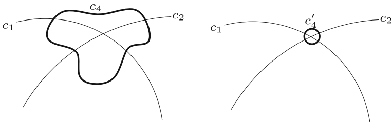
Fig. 8 When c_4 separates the two intersection points of c_1, c_2 and c_4 does not intersect c_3
