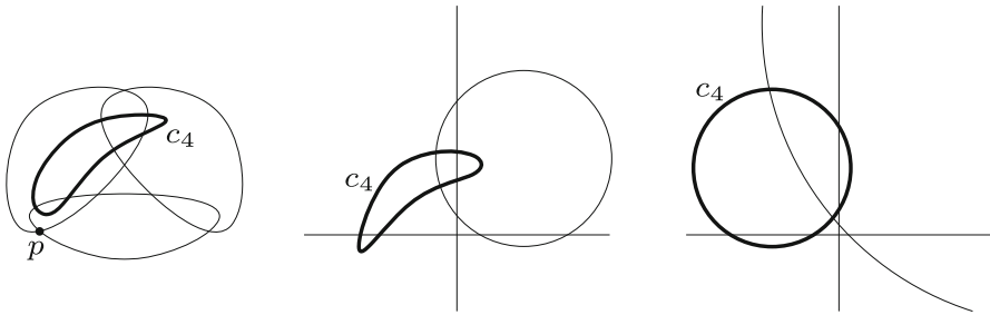
Fig. 17 The arrangement (c_1, c_2, c_3) is as in Fig. 6, right, and c_4 intersects two sides of a 2-face
