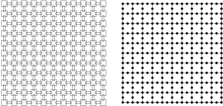
Fig. 25 The arrangement \mathcal{H} of convex pseudocircles and its intersection graph H
