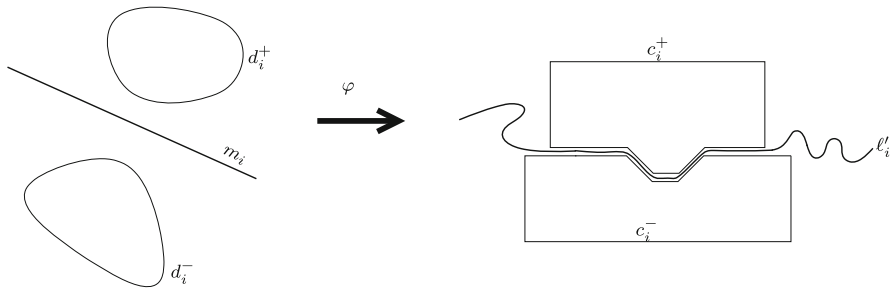
Fig. 36 A line m_i separating d_i^- and d_i^+ (left) and their images under \varphi (right)
