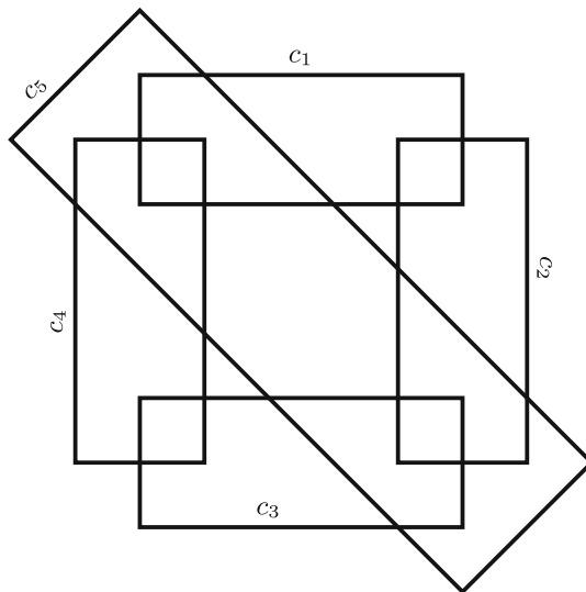
Fig. 1 An arrangement of five pseudocircles that is not circleable
