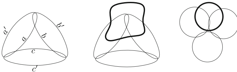
Fig. 9 The situation where (c_1, c_2, c_3) is equivalent to Fig. 6, right
