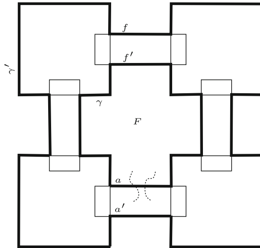
Fig. 29 The segments a, a', f, f' and the curves \gamma, \gamma'
