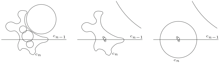
Fig. 5 If (c_1, \dots, c_{n-1}) is circleable and c_n intersects only one pseudocircle
