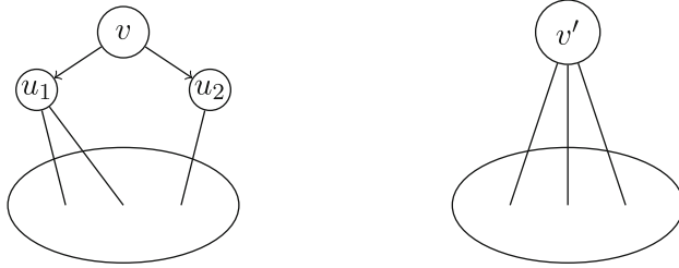
Fig. 5 a The graph G having a degree-2 vertex v with two neighbors u_1 and u_2 ; b the graph G' after deleting \{v, u_1, u_2\} and introducing the new vertex v'
