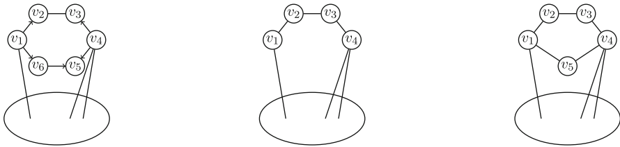
Fig. 10 a The graph G containing a 6-cycle v_1v_2v_3v_4v_5v_6 with four degree-2 vertices v_2, v_3, v_5 and v_6 ; b the graph G' after applying (1) in R10 on G ; c the graph G' after applying (2) in R10 on G
