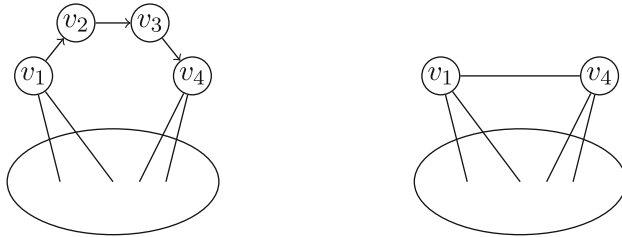
Fig. 6 a The graph G , where v_2 and v_3 are two adjacent degree-2 vertices; b the graph G' after deleting v_2 and v_3 and adding the edge v_1v_4
