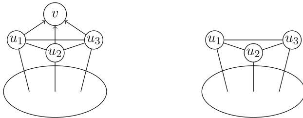
Fig. 4 a The graph G , where vertex v has a clique neighborhood and the weight of v is less than the weight of any neighbor of it; b the graph G' after deleting v from G and updating the weight w(u) := w(u) - w(v) for all u \in N_G(v)
