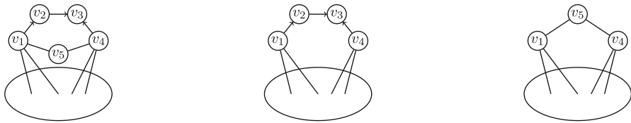
Fig. 9 a The graph G containing a 5-cycle v_1 v_2 v_3 v_4 v_5 with three degree-2 vertices v_2, v_3 and v_5 ; b the graph G' after applying (1) in R9 on G ; c the graph G' after applying (2) in R9 on G
