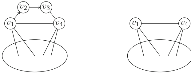
Fig. 7 a The graph G , where v_2 and v_3 are two adjacent degree-2 vertices in a 4-cycle v_1 v_2 v_3 v_4 ; b the graph G' after deleting v_2 and v_3 from G
