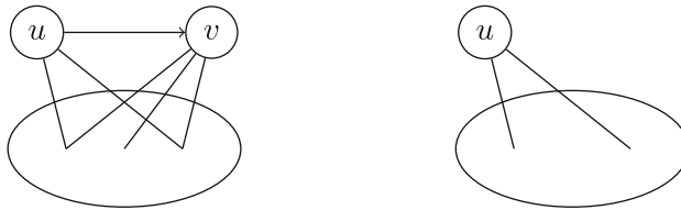
Fig. 2 a The graph G , where vertex v is dominated by vertex u , and v is removable; b the graph G' that is obtained from G by deleting the removable vertex v
