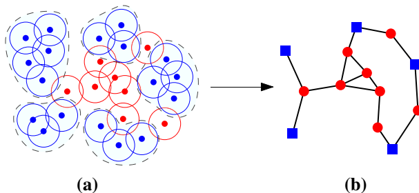
Fig. 4 An illustration of the component contraction; (a) red disks are Steiners and blue disks are terminals; (b) red vertices are Steiner vertices and blue vertices are contracted terminal components (Color figure online)
