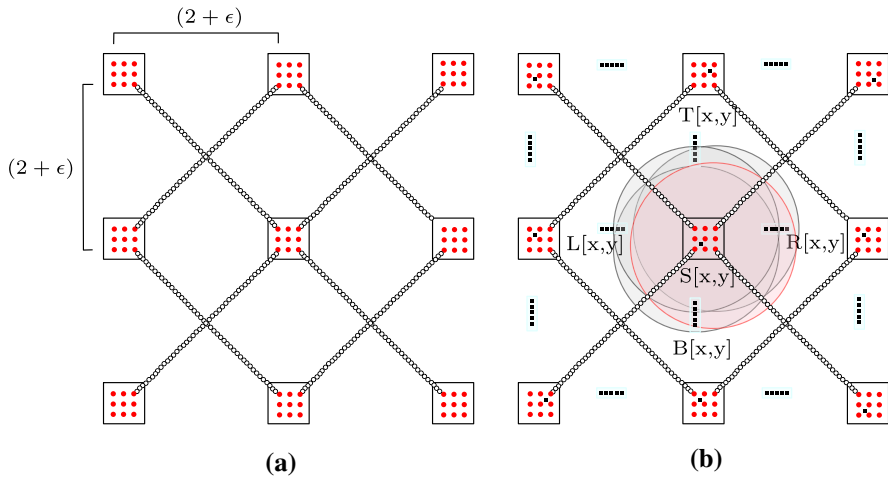
Fig. 5 (a) The schematic diagram of the cells, after adjusting the distance between adjacent cells which is 2 + \epsilon . The red disks inside each cells, are the coordinates where the center of the Steiner disk of radius 1 will be placed. The diagonal chains consisting of terminal disks of radius \kappa , are connecting the cells diagonally. (b) The small black dots inside each cell are extra terminals of radius \delta . Consider a cell S[x, y] . The shaded grey disks are the potential disks and the shaded red disk is chosen in the solution from D[x, y] (Color figure online)
