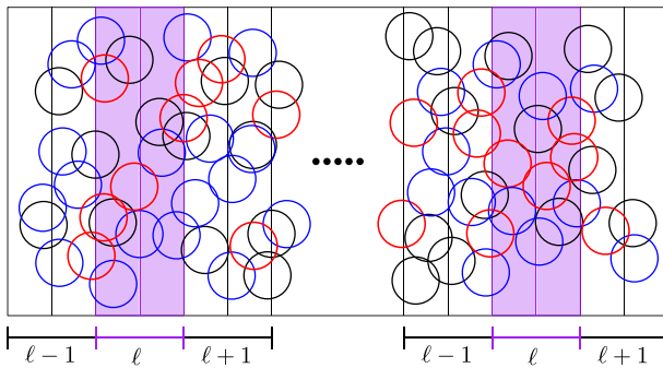
Fig. 3 An illustration of grid labelling. The blue disks are terminals, and the red and black disks are chosen Steiner vertices and not-chosen non-terminal vertices, respectively (Color figure online)
