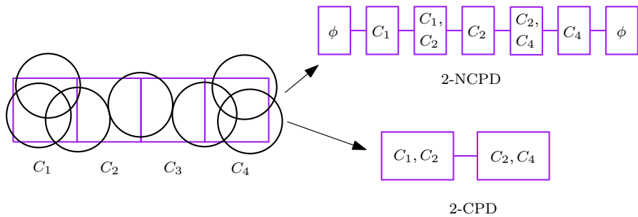
Fig. 1 An illustration of nice 2-clique path decomposition
