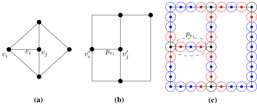
Fig. 2 (a) A planar graph G of maximum degree 4, (b) the intermediate rectilinear embedding G' of G , (c) the unit disk graph G_C ; the black disks are corresponding to the grid vertices of G' , the red disks are Steiner disks and the blue disks are the terminal disks (Color figure online)
