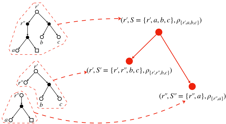
Fig. 4 The figure represents the encoding of a tree as a state tree. Each state is a succinct encoding of a tree that captures its boundary information (i.e. the portals). The state tree then encodes how a tree is further decomposed to subtrees. In the example we have a one-step decomposition – an allowable child-pair, and it corresponds to an 1-level state tree with three states
