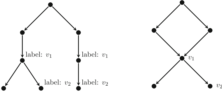
Fig. 2 Example of a multi-tree and corresponding subgraph of G
