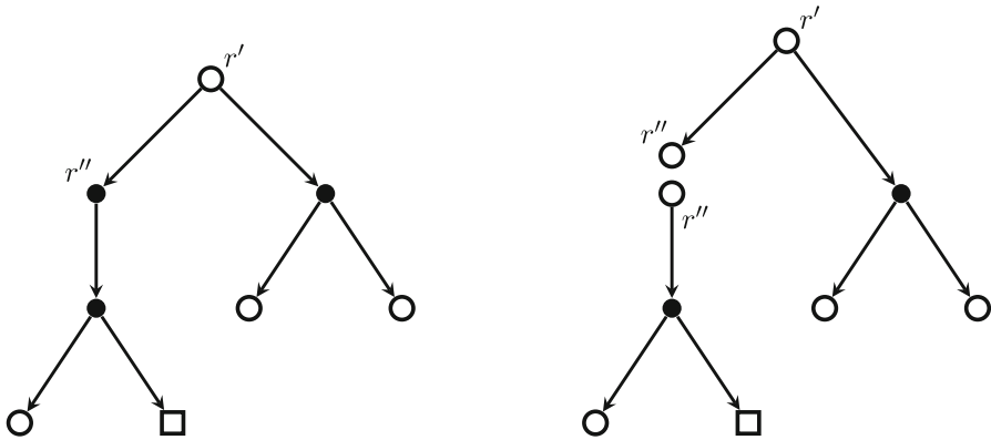
Fig. 3 Example of a subtree T' and the subtrees corresponding to an allowable child-pair. Portals are drawn as hollow circles and terminals as hollow squares. The left subtree is T' , the right subtrees are T'_1 (top-right) and T'_2 (bottom-right). The sets of portals S, S_1, S_2 contain the portals of T', T'_1, T'_2 respectively
