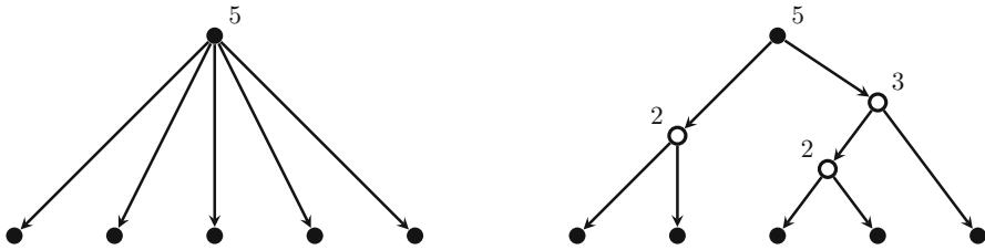
Fig. 1 Example of the transformation to a graph with out-degree 2. On the left, a star consisting of the outgoing edges of a vertex is presented; on the right, the transformed subgraph. Vertices that are added by the transformation are represented as hollow circles. Each non-leaf vertex is labeled by its computed original degree
