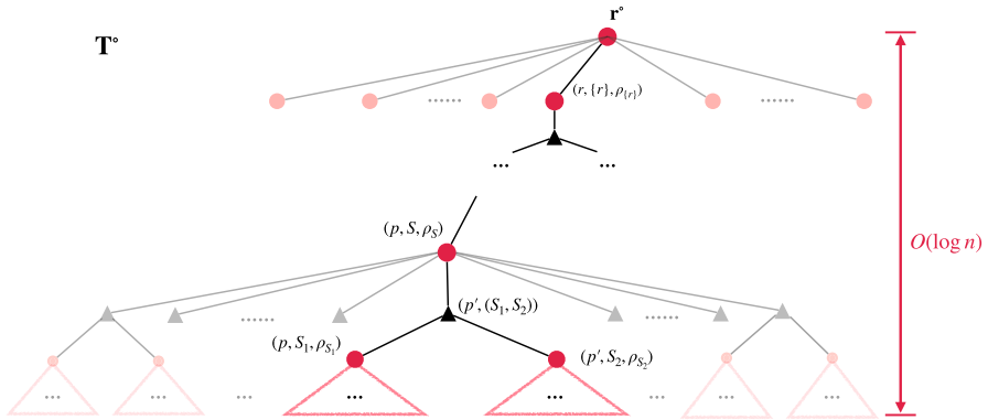
Fig. 5 T^\circ is the union of all good extended state trees. Virtual nodes are denoted as triangles, each of which represents a way to decompose (the subtree corresponding to) its parent state node. For example, (p', (S_1, S_2)) means we break the tree at vertex p' (thus creating a new portal p' ), and divide the portals S of the original tree (along with p' ) to the two new subtrees as S_1 and S_2
