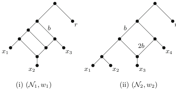
Fig. 3 Two weighted tree-child networks for which the maximum \mathcal{Q}_r -score is not realised by either a 0- or 1-reticulated cherry
