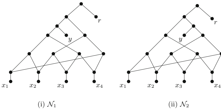
Fig. 4 In this figure all edges have weight 1. \mathcal{N}_1 and \mathcal{N}_2 are two non-isomorphic stack-free phylogenetic networks on \{x_1, x_2, x_3, x_4, y, r\} with the same multiset-matrix of inter-taxa distances
