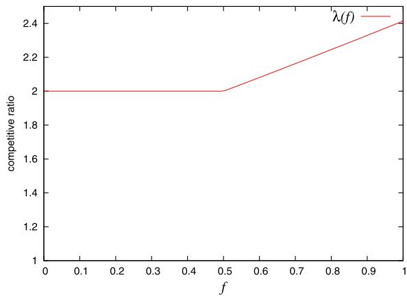
Fig. 1 The competitive ratio \lambda(f) for the proportional cost model
