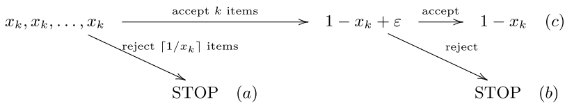
Fig. 5 The adversary for Lemma 12
