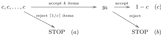
Fig. 6 The adversary for Lemma 13
