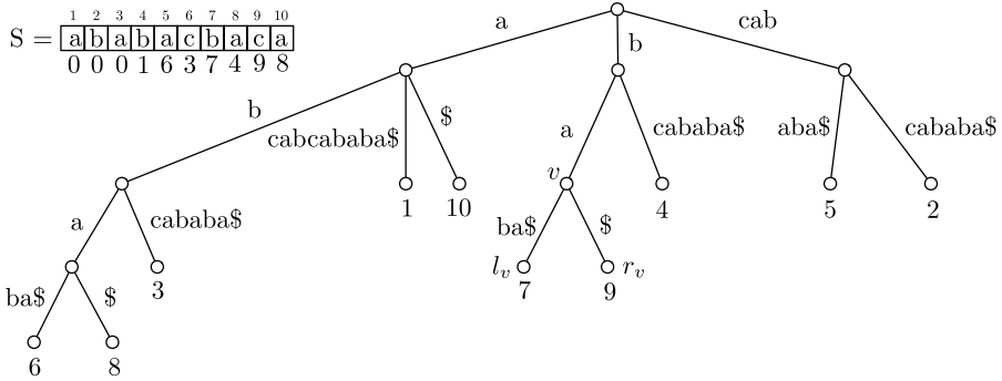
Fig. 1 A string S , the labeling for d = 2 (below the string), and the suffix tree of T_{SR} . Given a query P_1 = ab and P_2 = bac we find v = \text{locus}_{SR}(ba) (marked in the suffix tree). We have l_v = 6 and r_v = 7 from the left-to-right-order in T_{SR} . The substring range reporting query \text{REPORT}_S(P_2, 6, 7) returns 7. Hence, we report the occurrence at position 7 - 2 - 2 = 3
