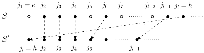
Fig. 2 Construction of the schedule S' . Packets from S are represented by circles: the ones included in S' are filled, the remaining ones are hollow. The packets from S' \setminus Q are not illustrated, since their assignment does not change with respect to X
