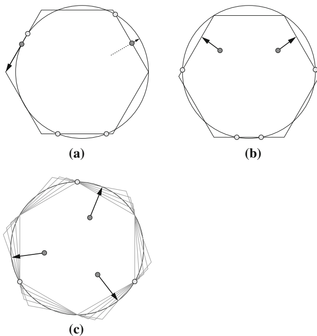
Fig. 9 (a) As the robot on the right moves to SEC, a Pre-regular configuration is accidentally formed. The robot on the left recognizes a Pre-regular configuration, and starts executing the corresponding protocol, which is inconsistent with the other robot's move. b To prevent this behavior, enough critical points are added. Now the swarm is guaranteed to stop as soon as a Pre-regular configuration is formed. c A case in which infinitely many Pre-regular configurations are formable. Still, only the innermost is relevant, because it can be reached before all the others
