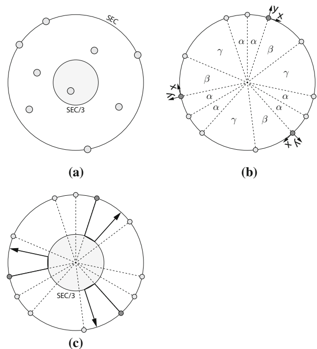
Fig. 2 a A swarm of robots, with its SEC and SEC/3. b The three highlighted robots form an analogy class. If their axes are oriented as indicated, the three robots have the same view. c The three dark-shaded robots are selected as walkers, and move according to the arrows. At the end of the move, each walker has an angular distance of \pi/3 (which is a multiple of 2\pi/n ) from a non-walker
