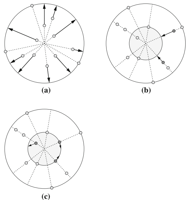
Fig. 3 a All robots move radially to reach SEC. b The most internal co-radial robots move radially to SEC/3. c When they are in SEC/3, they make a small lateral move
