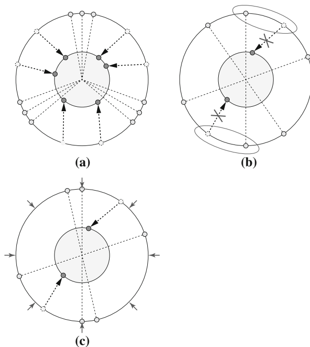
Fig. 8 a The principal relocation of the internal robots. b If the principal relocation is a proper subset of an analogy class, it cannot be the original position of the internal robots, or else a larger set of walkers would have been selected. c If the principal relocation forms an analogy class, it is used to determine the target set. Such targets remain fixed as the internal robots move within their respective sectors
