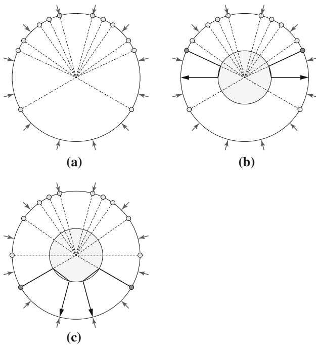
Fig. 6 a A locked configuration: the topmost robots are satisfied, the bottommost robots are non-movable, and all other robots would create co-radialities in the process of reaching their targets. b A preliminary move is made to unlock the configuration. c When the configuration is unlocked, the bottommost robots become movable
