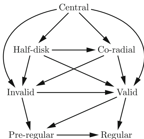
Fig. 11 Possible transitions between configurations of Algorithm UCF
