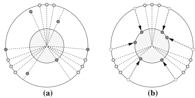
Fig. 7 Two types of Valid configurations. a Some analogous robots lie between SEC and SEC/3, and all other robots are on SEC. b All robots are on SEC or on SEC/3, and the distribution of the internal robots is compatible with a possible initial configuration in which they were all on SEC, forming an analogy class
