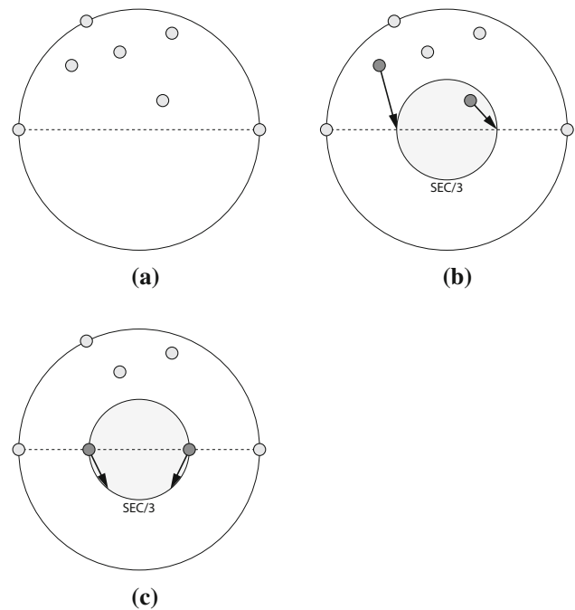
Fig. 4 a A Half-disk configuration, with the principal line. b Two robots move to the intersection between the principal line and SEC/3 . c The same two robots move to the non-occupied half-disk
