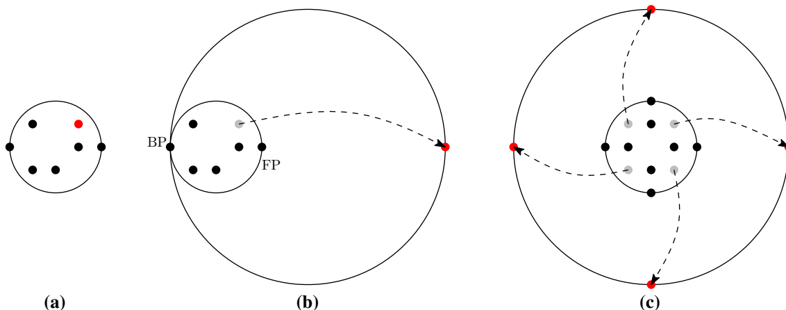
Fig. 2 a An asymmetric configuration of robots and the smallest enclosing circle. b A bi-circular configuration formed by moving one of the robots. c An \text{SCC}(q) configuration with q = 4
