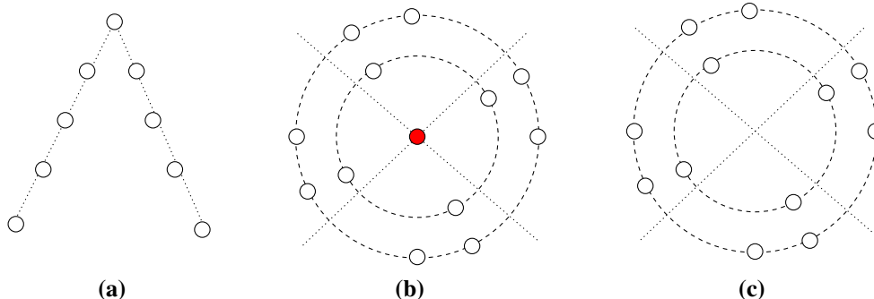
Fig. 1 A configuration \gamma where robots occupy distinct locations, such that: a the symmetricity \rho(\gamma) = 1 and each robot has a distinct view; b the symmetricity \rho(\gamma) = 1 and only one robot (the shaded one) has a unique view; c the symmetricity \rho(\gamma) = 4 and no robot has a unique view
