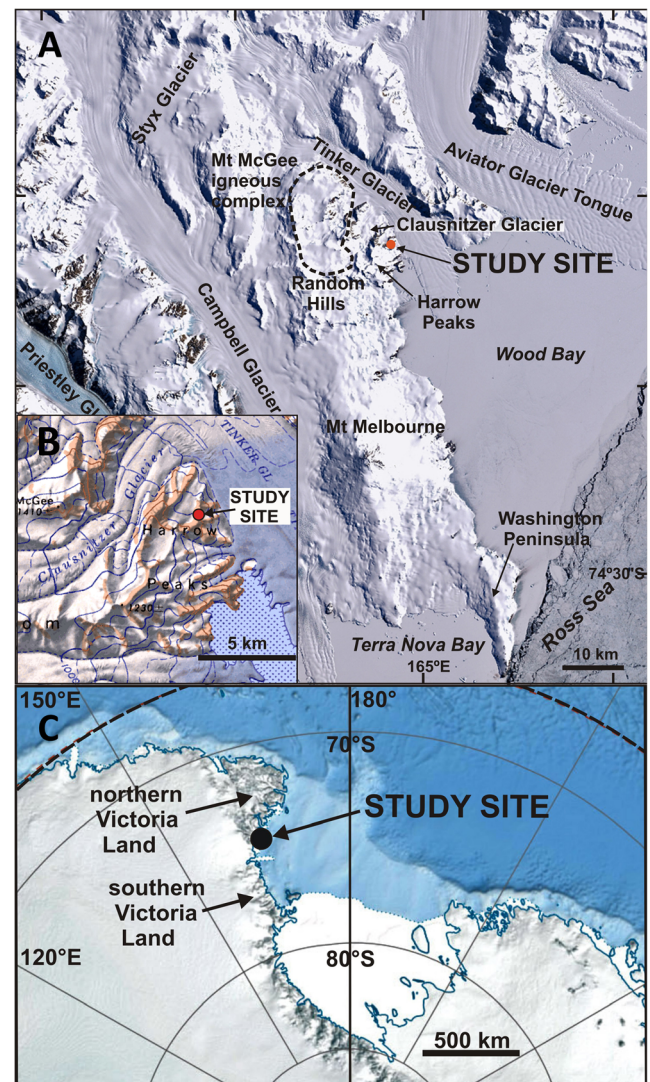
Fig. 1 Satellite images showing the location of the study area, Harrow Peaks, in northern Victoria Land, Antarctica, and localities mentioned in the text. Topographical base map used in B from USGS (1967)
