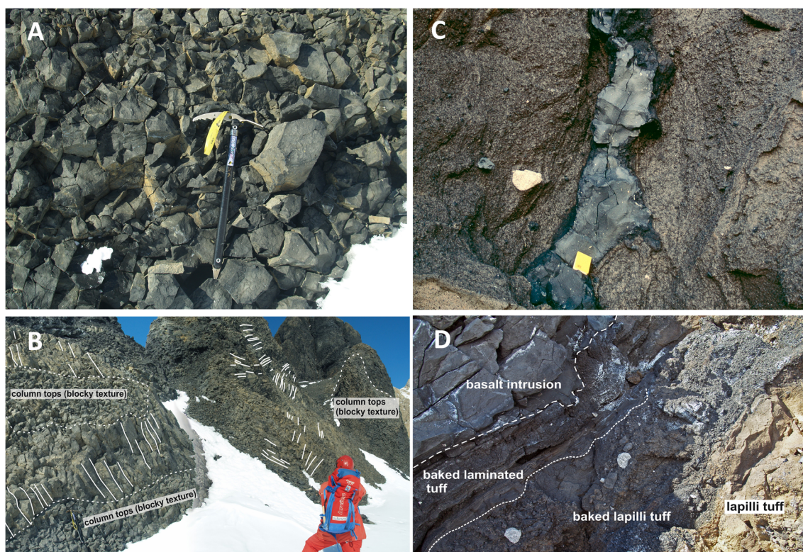
Fig. 6 Views of the coherent lithofacies. a Blocky jointing in the basalt plug; the ice axe is 60 cm long. b Entablature (also known as kubbaberg) prismatic jointing in the basalt plug; selected prismatic joints shown by white lines to highlight orientation variations. c Thin dyke intruding
