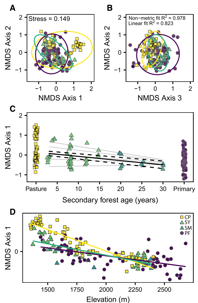
Fig. 2 Non-metric multidimensional scaling (NMDS) ordination of standardised species composition within primary forest and pasture habitats (a, b). Ellipses represent 95% confidence intervals for each habitat type. NMDS axis 1 scores against habitat type with a linear regression of secondary forest age (c). Regression line plotted with predicted values from elevation model, with 95% confidence interval (CI) represented by dashed lines. Grey lines show fitted slopes for the interaction between secondary forest age and elevation, from low (top) to high (bottom) elevations. NMDS axis 1 scores plotted against elevation (m), by habitat type: cattle pasture (CP), young (SY) and mature (SM) secondary, and primary (PF) forest (d)
