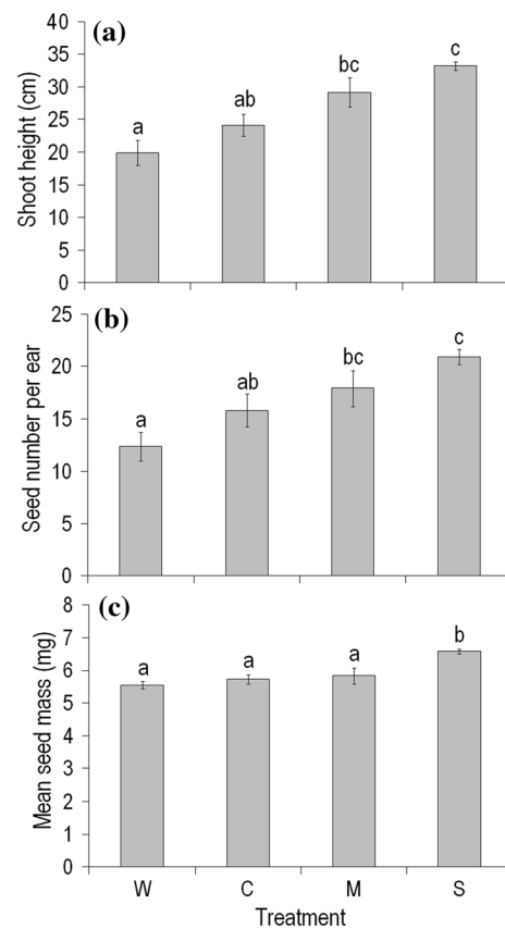
Fig. 2 Effects of the previous-year (2015) rainfall manipulations on a maximum vegetative shoot height (cm), b seed number per ear, and c mean single seed mass (mg) of Secale sylvestre growing in the plots of the field experiment in 2016 (maternal generation). Values are treatment mean \pm SE ( n=6 ). Treatment symbols are defined in the legend of Fig. 1. Different letters above the bars indicate significant ( P<0.05 ) differences between treatments. Results of Tukey’s HSD tests following general linear mixed models are shown
