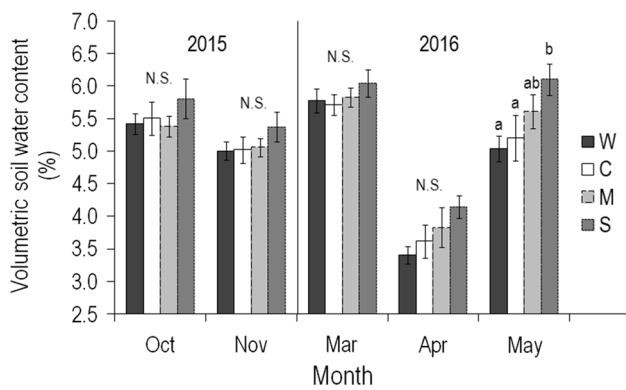
Fig. 1 Effects of rainfall manipulations on volumetric soil water content (%) at 0–30-cm depth in the plots of the field experiment during the period of growth and reproduction of the studied Secale sylvestre plants (maternal generation). Values are treatment mean \pm SE ( n=6 ) in each month. Treatments are watering (W), control (C), moderate drought (M), and severe drought (S). Different letters above the bars denote significant ( P<0.05 ) differences, while N.S. indicates the lack of significant differences between treatments within each month separately. Results of Tukey’s HSD tests following two-way repeated-measures ANOVA are shown
