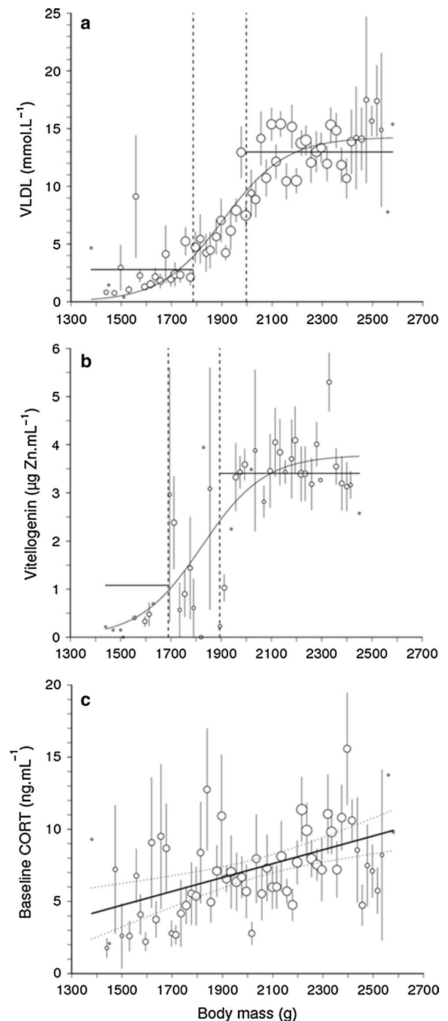
Fig. 2 Relationship between total VLDL (a), vitellogenin-VTG (b) and baseline CORT (c) with body mass at capture. Logistic regression are fitted (solid black lines) as well as sections (dashed vertical lines) with horizontal black lines indicating the mean for the identified sections. Values are mean \pm SEM. Dot sizes are proportional to \log(n)
