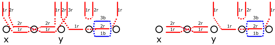
Fig. 2 We suppose that N = 2 , we represent the colour 1 by blue and the colour N = 2 by red, we assume that \mathcal{G} is a connected subset of \mathbb{Z} with five vertices and edges connecting nearest neighbour vertices and the vertical links are on edges connecting the vertices of \mathcal{G} to g , the ghost vertex is not represented in the figure. Left : A configuration w \in \mathcal{S}^N(\{x, y\}) such that M_{x,y}(w) = 2 (see the definitions in the proof of Lemma 2.5). Right : A configuration F_N(w) , which is obtained from w by removing the extremal links of the two (\{x, g\}, \{y, g\}) -extremal walks and by leaving unpaired the links to which such external links were paired
