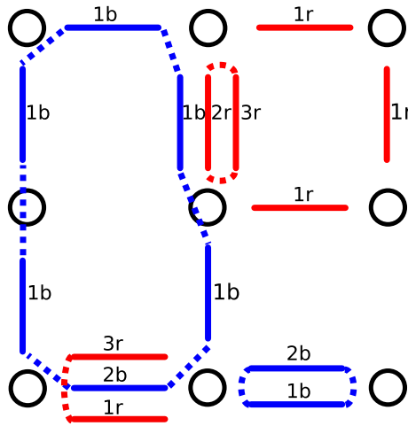
Fig. 1 A configuration w = (m, c, \gamma) \in \mathcal{W}_{\mathcal{G}} , where \mathcal{G} corresponds to the graph \{1, 2, 3\} \times \{1, 2, 3\} with edges connecting nearest neighbours and the lowest leftmost vertex corresponds to (1, 1) . On every edge e , the links are ordered and receive a label from 1 to m_e . In the figure, the numbers 1, 2, ... are used for the identification of the links and the letters b and r are used for the colours which are assigned to the links by c (we assume that N = 2 and that each link might be either blue or red). Paired links are connected by a dotted line. For example, the first link on the edge connecting the vertices (1, 1) , (2, 1) is coloured red, it is paired at (1, 1) with the third link on the same edge and it is unpaired at (2, 1) . Moreover, both links touching the vertex (3, 3) are red and they are unpaired at (3, 3) . Finally, no link is on the edge which connects the vertices (1, 2) and (2, 2)
