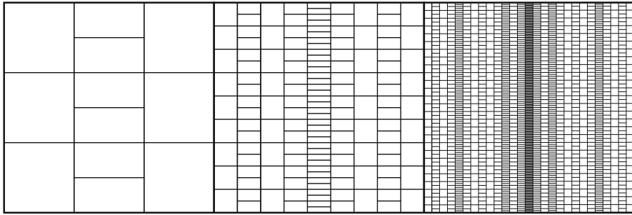
Fig. 4 The tiling \mathbf{H}^1 \mid \mathbf{H}^2 \mid \mathbf{H}^3
