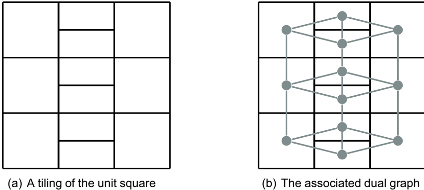
Fig. 1 Tilings and their dual graph
