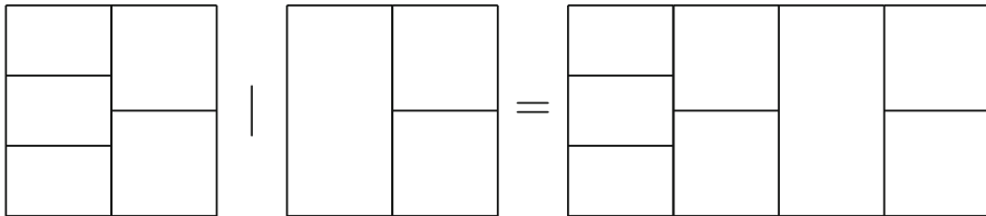
Fig. 3 An example of the tiling concatenation S | T
