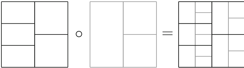
Fig. 2 An example of the tiling product S \circ T
