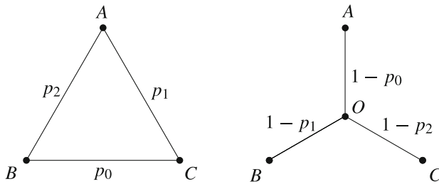
Fig. 7 The star–triangle transformation
