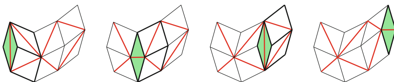
Fig. 10 A new rhombus is introduced on the left (marked in green ). This is then ‘slid’ along the pair of tracks by a sequence of star–triangle transformations, until it reaches the right side where it is removed
