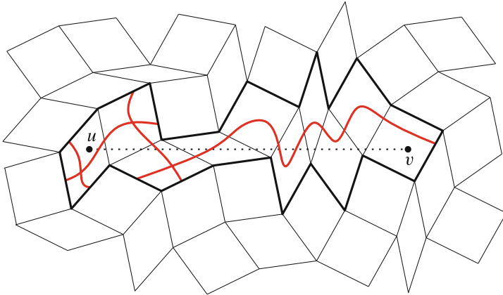
Fig. 5 The region U_{uv}^N is outlined in bold, and contains a chain of cells joining u to v . The events H_k are drawn explicitly for the first two contiguous pairs of cells
