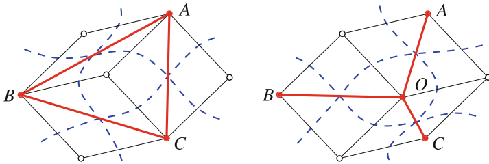
Fig. 9 The triangle on the left is replaced by the star on the right. The new vertex O is the circumcentre of the three dual vertices of the surrounding hexagon of G^\diamond
