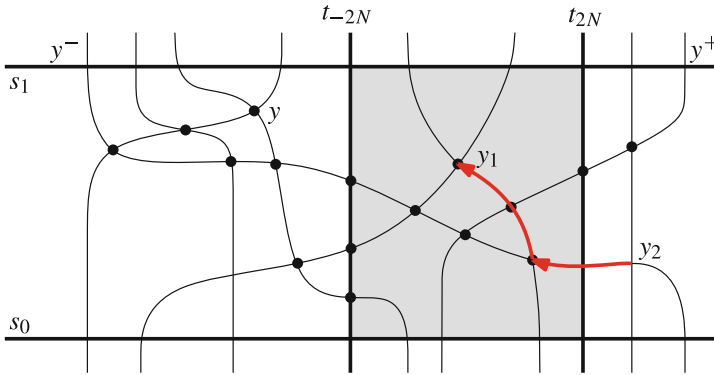
Fig. 20 The black points are indicated. The path \gamma from y_2 to y_1 is drawn in red. The points y and y_1 are maximal, and are not comparable. The region \mathcal{R} is shaded
