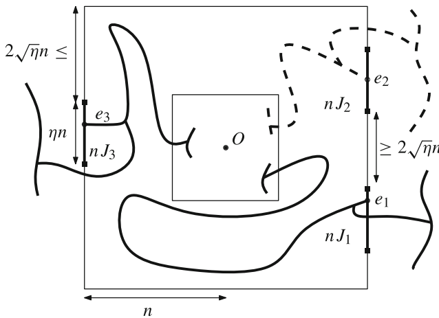
Fig. 23 The event A_{\sigma}^{J,J}(N, n) with \sigma = (1, 0, 1) and \eta -landing-sequence J . Each crossing \Gamma_i is an \eta -fence with exterior endpoint e_i \in nJ_i
