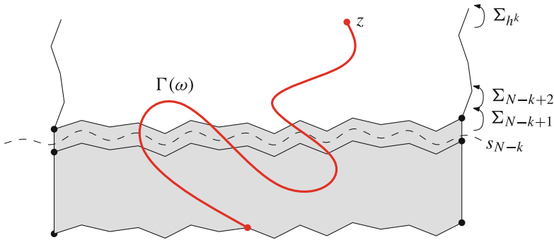
Fig. 18 The transformation V_k moves s_{N-k} upwards by N units
