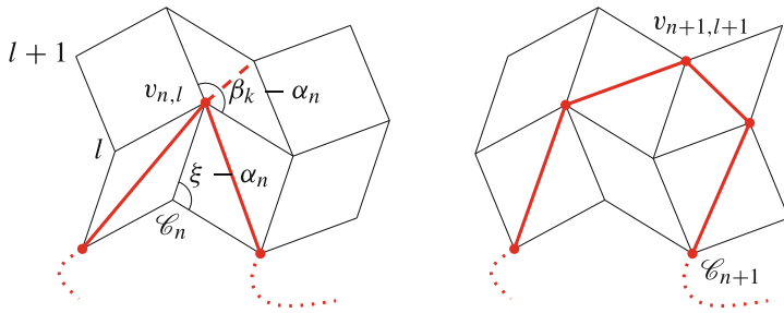
Fig. 17 The third case of Fig. 11. If the dashed edge in the initial configuration (left) is open then, with probability \eta_k(n) , the resulting configuration is that on the right side
