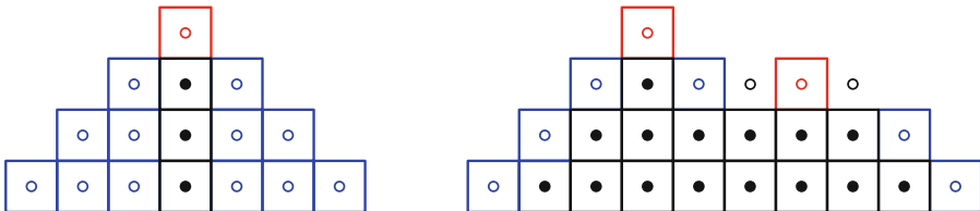
Fig. 14 Left One step in the evolution of \mathbf{H} . The initial range \mathbf{H}^0 has only one occupied column (black). The blue/black squares form the mountain of the black column. The red square is added at random. Right One step in the evolution of the \mathbf{X}^k (or \mathbf{H}^k when regular). The black squares are the configuration at step k , the blue squares are the additions at time k + 1 due to the covering, and the red squares are the random additions
