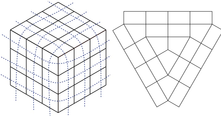
Fig. 3 Part of a rhombic tiling without the square-grid property, and one of the two corresponding isoradial graphs
