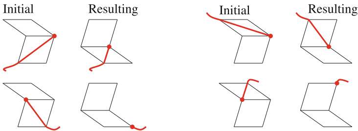
Fig. 12 If an endpoint of \gamma lies between the two tracks, the corresponding edge is sometimes contracted to a single point
