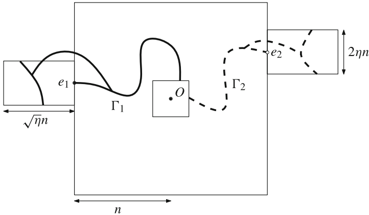
Fig. 22 A primal \eta -exterior-fence \Gamma_1 with exterior endpoint e_1 , and a dual \eta -exterior-fence \Gamma_2
