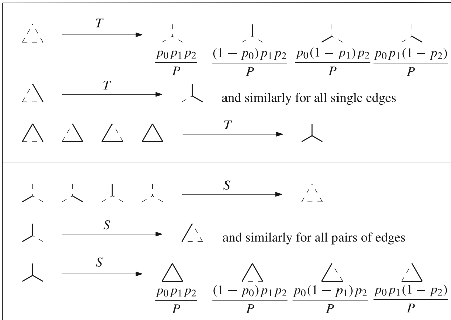
Fig. 8 The random maps T and S . Note that P := (1 - p_0)(1 - p_1)(1 - p_2)
