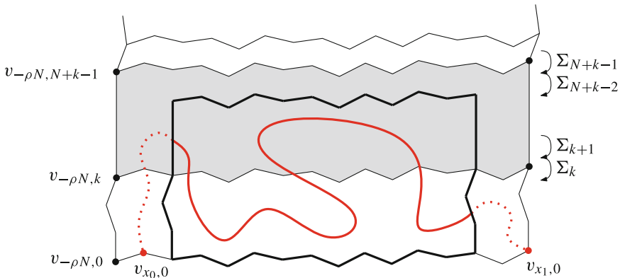
Fig. 13 The transformation U_k raises the (shaded) regular block by one unit, and moves the track above by N units downwards
