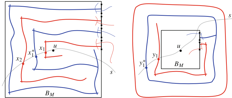
Fig. 24 Left The event H_M for k = 4 . The red paths are open, the blue paths are open*. The thin coloured paths are parts of the interior fences of A_k^{J,J}(M, m) . Right The event K_M for k = 2 , together with parts of the exterior fences of the arm-event. The track s intersects the open/open* crossings just above the points labelled x_i and y_i
