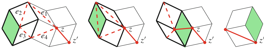
Fig. 19 Three star-triangle transformations contributing to \Sigma_{j+1} , from left to right. The dashed edges are closed, the bold edges are open. The first and last passages occur with probability 1, and the second with probability p_{e_1} p_{e_4} / (1 - p_{e_1})(1 - p_{e_4})
