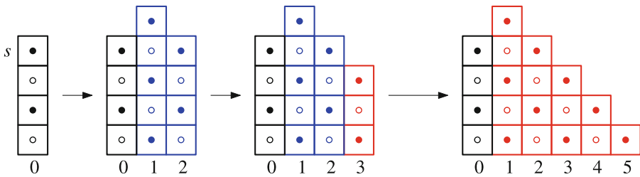
Fig. 15 An illustration of the sequence \tilde{\mathbf{L}}(0, s)^j beginning with the initial column \tilde{\mathbf{L}}(0, s)^{N+k} = \Delta(0, s) . This column is unchanged up to and including j = s , and then it evolves as illustrated
