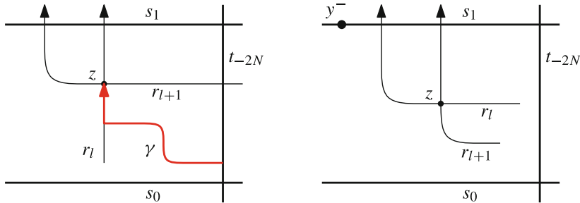
Fig. 21 Left The oriented track r_{l+1} crosses r_l from right to left, in contradiction of the choice of \gamma as highest. Right The track r_{l+1} crosses r_l from left to right
