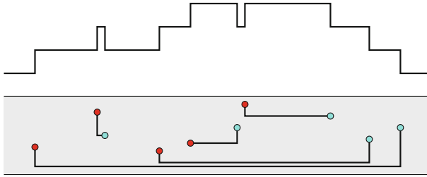
Fig. 2 The random walk F associated with red and blue points in the strip, and the matching with disjoint arcs from the proof of Theorem 1(iv) (color figure online)
