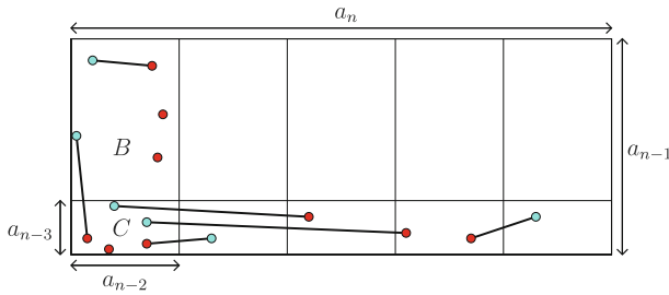
Fig. 4 An n -block A , its children including its heir B , and their heirs including B 's heir C . Also shown are the new edges added in stage n assuming A is neither bad nor dodgy
