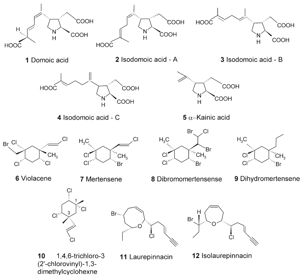
Fig. 1 Chemical structure of insecticidal seaweed compounds (1–12) isolated from Chondria armata , Digenea simplex , Laurencia pinnata , L. papillosa , Plocamium cartilagineum , and P. telfairiae
