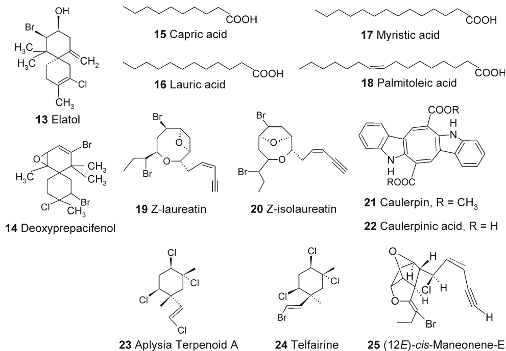
Fig. 2 Chemical structure of mosquito larvicidal seaweed compounds ( 13–25 ) isolated from Cladophora glomerata , Caulerpa racemosa , Laurencia dendroidea , L. nipponica , L. papillosa , and Plocamium telfairiae
