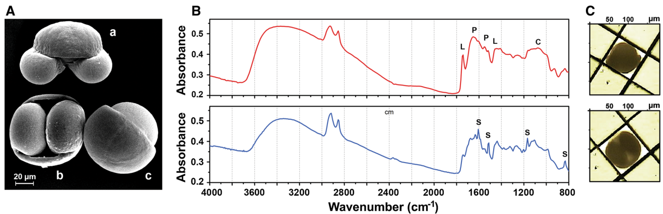
Fig. 2 Influence of spatial orientation of pollen samples on their infrared spectra. a SEM image of the intact Abies cephalonica pollen grains in: a equatorial front view, b distal polar view, and c equatorial profile view. b Global \mu FTIR spectra of single pollen grains with equatorial profile orientation ( red ), and distal polar orientation ( blue );
