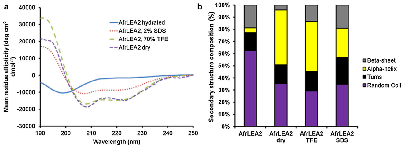
Fig. 2 Left panel CD spectra for recombinant AfrLEA2 in the hydrated state, in the presence of 2 % SDS, 70 % TFE, and after desiccation. Right panel secondary structure composition of
