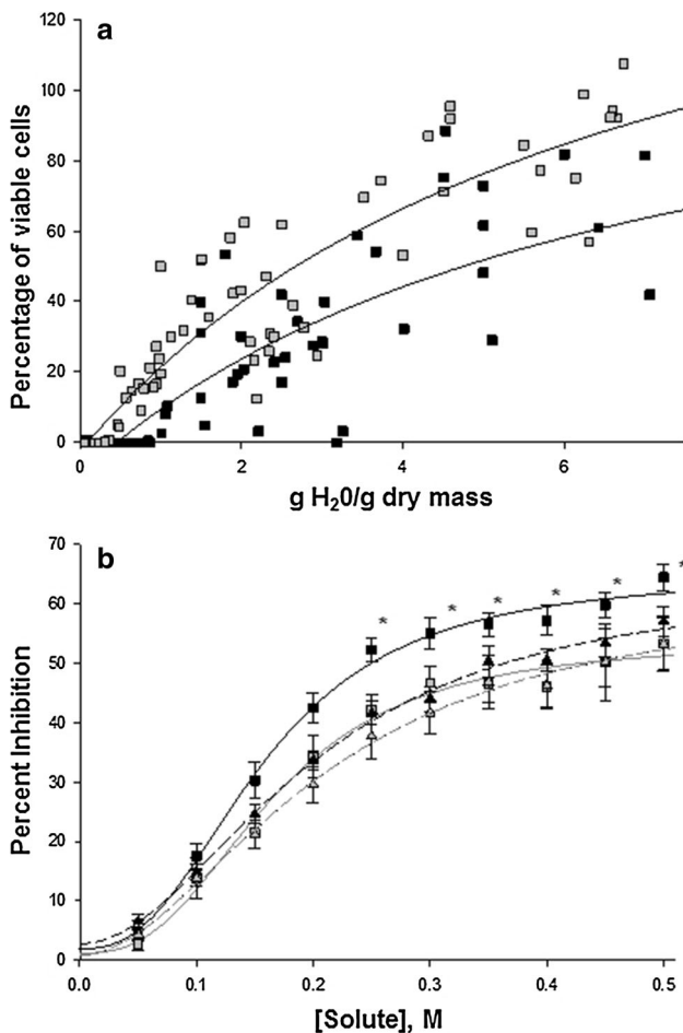
Fig. 5 a Viability of Kc167 cells from Drosophila melanogaster after drying and rehydration. Kc167 control cells (black) and cells expressing AfLEA1.3 (gray) were convectively dried in a solution containing 200 mM trehalose. Expression of AfLEA1.3 significantly improved the cellular response to desiccation (ANCOVA: F_1 , P < 0.0001 , r^2 = 0.74 ). b Percent inhibition of respiration in permeabilized Kc167 control cells (square, solid line) and Kc167-AfLEA1.3 cells (triangle, dashed line) measured at various concentrations of NaCl (black) or KCl (gray, dashed line). Oxygen consumption was measured in presence of malate, glutamate, pyruvate, succinate and ADP ( n = 4 , \pm SE). *Significant differences between cell lines ( P \leq 0.05 ) (redrawn from Marunde et al. 2013)
