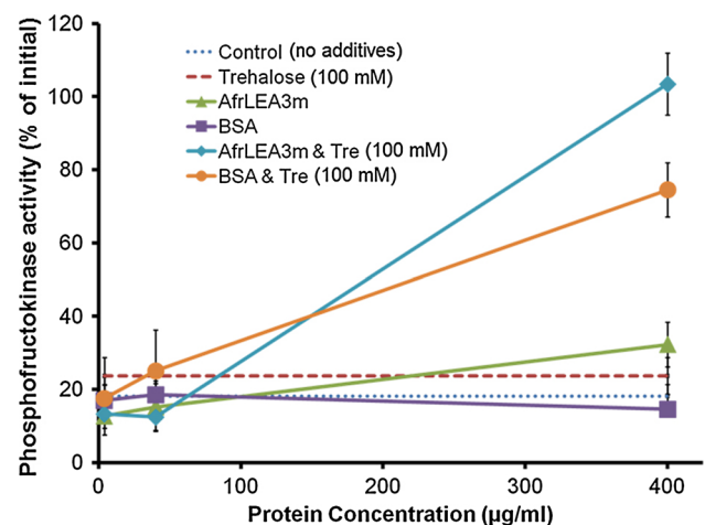
Fig. 3 Residual PFK activity after desiccation without additives (control) or in the presence of protectants. Values are reported as percent of the initial PFK activity measured prior to desiccation (mean \pm SD, n = 9 ). AfrLEA3m plus trehalose provided a significantly higher level of protection than did any other treatment (one-way ANOVA plus Tukey, P \leq 0.05 ) (redrawn from Boswell et al. 2014b)
