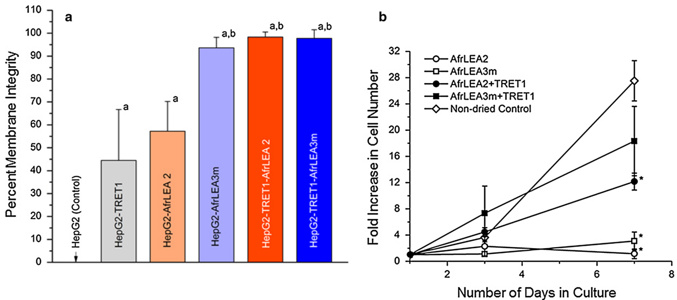
Fig. 6 Membrane integrity and long-term growth of HepG2 cells after spin-drying and immediate rehydration. a Control cells contained no intracellular trehalose or LEA proteins. HepG2-TRET1 cells contained approximately 20 mM trehalose; HepG2-AfrLEA2, expressed AfrLEA2 but without intracellular trehalose; HepG2-AfrLEA3m, expressed AfrLEA3m but without intracellular trehalose; HepG2-TRET1-AfrLEA2, expressed AfrLEA2 and contained intracellular trehalose; HepG2-TRET1-AfrLEA3m expressed AfrLEA3m and contained intracellular trehalose. All treatments were dried with extracellular trehalose present. Membrane integrity was determined using Syto-13 and ethidium bromide viability dyes. Values are mean \pm SD ( n = 3 –9 independent determinations). “a” indicates
