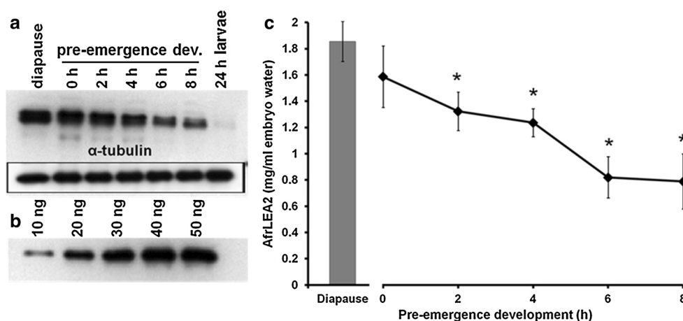
Fig. 1 Measurements of AfrLEA2 protein in extracts of A. franciscana by Western blot analysis. a Expression for AfrLEA2 is shown at various stages of the life cycle [diapause; pre-emergence development (hours 0, 2, 4, 6, and 8); and nauplius larvae (24 h)]. \alpha -Tubulin was used as a loading control. b Concentration dependency of
