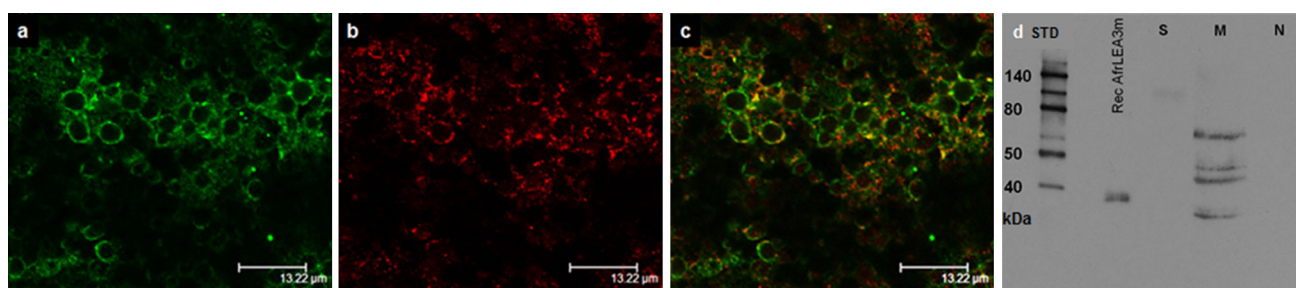
Fig. 4 Subcellular localization of AfrLEA3m (and its closely related isoforms recognized by AfrLEA3m antibody) in embryos of A. franciscana visualized with confocal microscopy. Shown are the images for AfrLEA3m proteins ( a green), VDAC ( b red) and the merged image ( c yellow) indicating areas of co-localization. d Immunoblot of AfrLEA3m for the supernatant (S), mitochondrial
