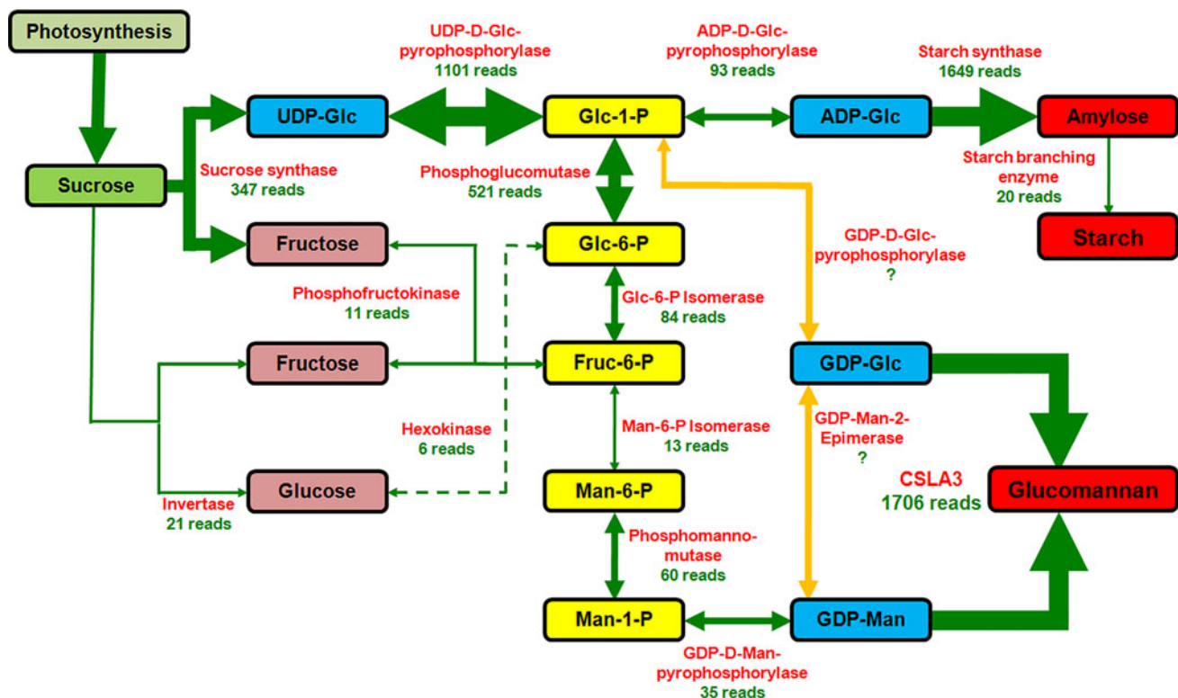
Fig. 4 Proposed glucomannan and starch biosynthesis pathway in the A. konjac corm based on the established EST database. Presented is the nucleotide sugar interconversion pathway from sucrose to GDP-mannose and GDP-glucose, the two building blocks of glucomannan as well as the starch biosynthesis pathway. The necessary converting enzymes found in the EST data are given in red with the number of obtained reads in green. The thickness of the arrows is representative
