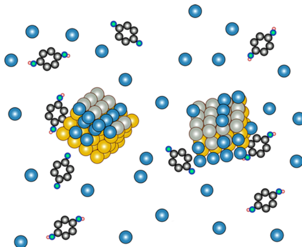
Fig. 3 “Camera lucida” representation of the autometallographic process. When the hydroquinone molecules (hexagonal molecules, being the reductor molecules of the AMG developer) adhere to the gold quantum dots ( stained gold ), electrons are released into the QD, and this event builds up energy in the valence cloud that forms the attraction forces of the nanocrystal. The higher energy level brought about by the surplus electrons increases the statistical probability that silver ions ( stained blue ) that have attached themselves to the nanocrystal lattices of the IQ dots catch an electron and are turned into a silver atom ( stained silver in the drawing). The “new” silver atom shares valence electrons with the valence cloud of the original nanocrystals and is therefore a genuine part of the original gold quantum dot. When the AMG enhanced QD’s have reached the most optimal size for electron, respectively, light microscopic analysis the process is stopped by the developer being replaced by a 5% sodium thiosulphate solution that removes silver ions from the section. Proton-induced X-ray emission spectroscopic analysis ( PIXE ) of the tissue surrounding gold implants confirms that gold ions are liberated, i.e. that the AMG observations are valid (Danscher 2002; Danscher et al. 1984)
