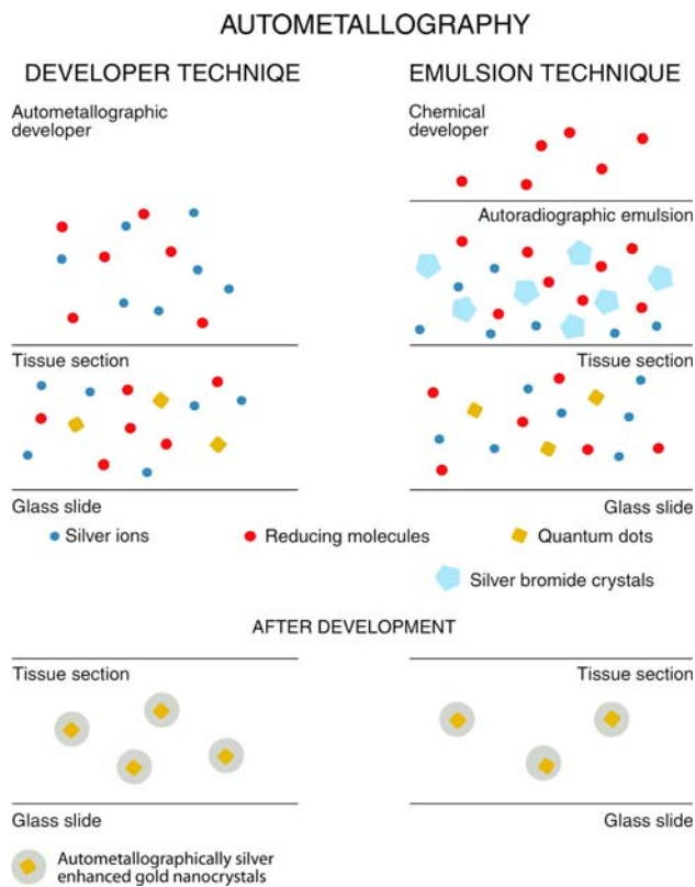
Fig. 4 Autometallographic enhancement of gold nanoparticles can be performed in two different ways. To the left an AMG solution is poured into jars containing glass slides with the tissue sections, or the AMG developer is dripped directly onto the individual section. To the right the slides are first dipped into an autoradiographic emulsion, allowed to dry for 10 min and then placed in jars filled with a common chemical developer. Both approaches result in the tissue sections being permeated with a solution of reducing molecules and silver ions. As the gold nanocrystals in the tissue sections catalyse the reduction of silver ions to metallic silver on their surfaces either of the techniques will result in the gold quantum dots/gold nanocrystals becoming encapsulated in metallic silver and thereby made visible at EM and LM levels, i.e. the gold nanoparticle has graphed its own position in the tissue section (modified from Danscher and Stoltenberg 2006)
