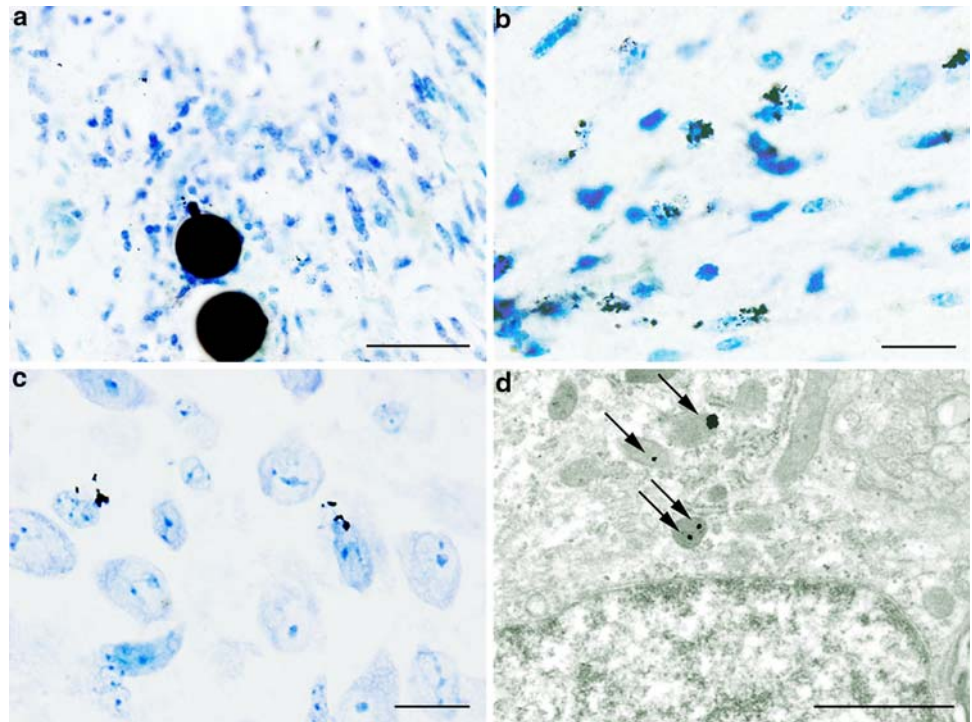
Fig. 1 Micrographs of 25 \mu\text{m} gold particles in cryo-lesioned neocortex containing tiny autometallographic (AMG) grains in adjacent cells. The grains result from AMG enhancement of gold nanoparticles created by accumulation of the bio-released gold ions in lysosomes. a 30- \mu\text{m} -thick cryo section showing two AMG enhanced gold particles in the inflammatory cerebral tissue. Scale bar 50 \mu\text{m} . b A neighbour section to section in a , but at a higher magnification. Note the heavy load of gold particularly in glia cells. Scale bar 20 \mu\text{m} . c High magnification of the cellular uptake of bio-released gold ion in a semi-thin Epon section. Scale bar 10 \mu\text{m} . d Electron micrograph of AMG silver enhanced gold ions located in lysosomes (arrows). Scale bar 1 \mu\text{m}
