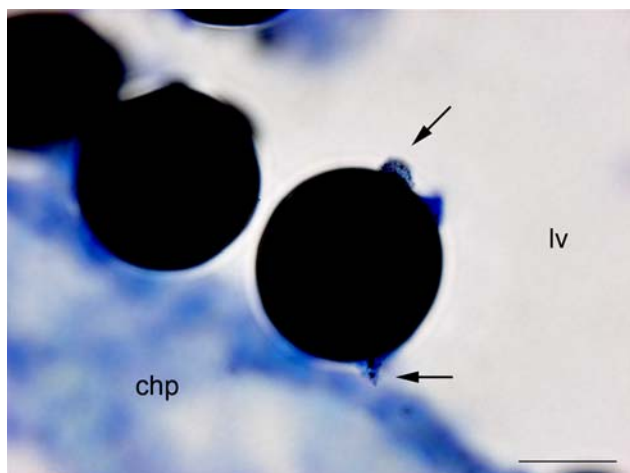
Fig. 2 Micrograph of AMG stained section of a mouse brain showing gold particles with adhering dissolucytotic macrophages in the lateral ventricle. The particles were injected 14 days before the mouse was killed. chp Choroid plexus, lv lateral ventricle, arrows macrophages loaded with bio-released gold
