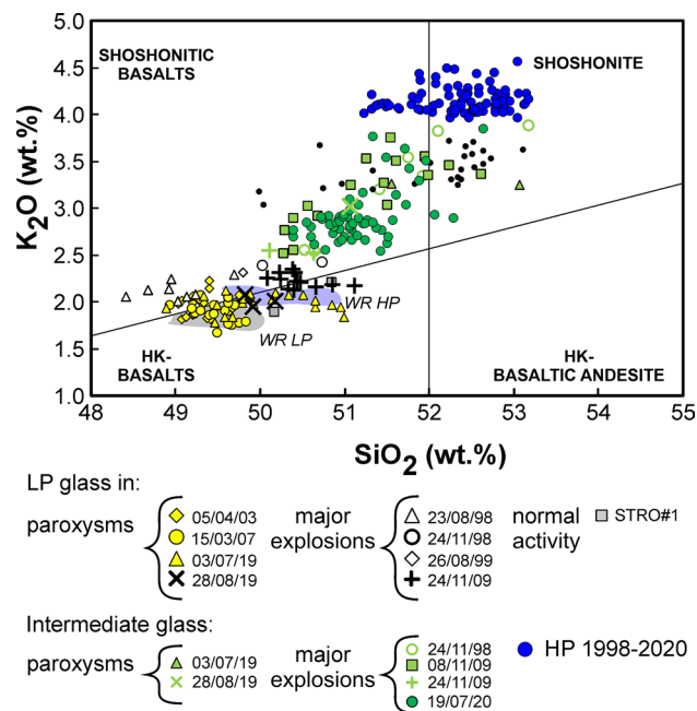
Fig. 1 Glass composition of the explosive products erupted in the period 1998–2020 plotted in the \text{SiO}_2 vs \text{K}_2\text{O} classification diagram (Peccerillo and Taylor 1976). The whole rock (WR) compositions from Métrich et al. (2001, 2005), Bertagnini et al. (2003), Landi et al. (2004, 2009) are reported for comparison as fields of variation (LP: gray; HP: blue). Black dots: 9 January 2005, data from Landi et al. (2009)
