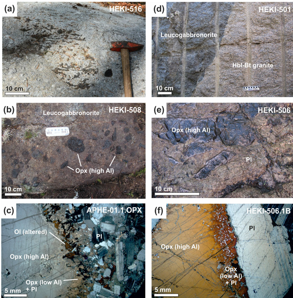
Fig. 2 a A typical sparsely plagioclase-porphyrific Ahvenisto leucogabbronorite with a coarse-grained raft of intergrown megacrystic orthopyroxene and plagioclase (observation HEKI-516). b Individual type 1 HAOMs on outcrop HEKI-508. c A photomicrograph (cross-polarized light) of a type 1 HAOM with a well-pronounced corona rim against the host leucogabbronorite (sample APHE-01.1.OPX). d Equigranular Ahvenisto Hbl-Bt (rapakivi) granite (on the right) cross-
