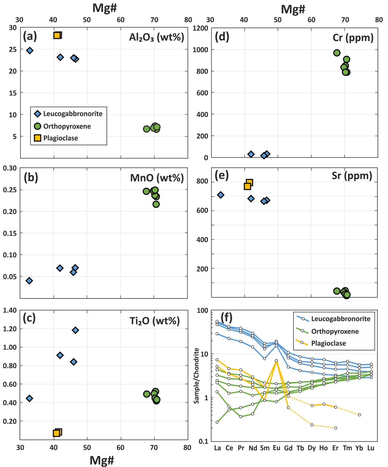
Fig. 4 Selected major- and trace-element variation diagrams for the bulk samples. a Mg# v. Al 2 O 3 (wt%), b Mg# v. MnO (wt%), c Mg# v. TiO 2 (wt%), d Mg# v. Cr (ppm), e Mg# v. Sr (ppm), and f chondrite-normalized REE abundances. Normalizing values from Boynton (1984)
