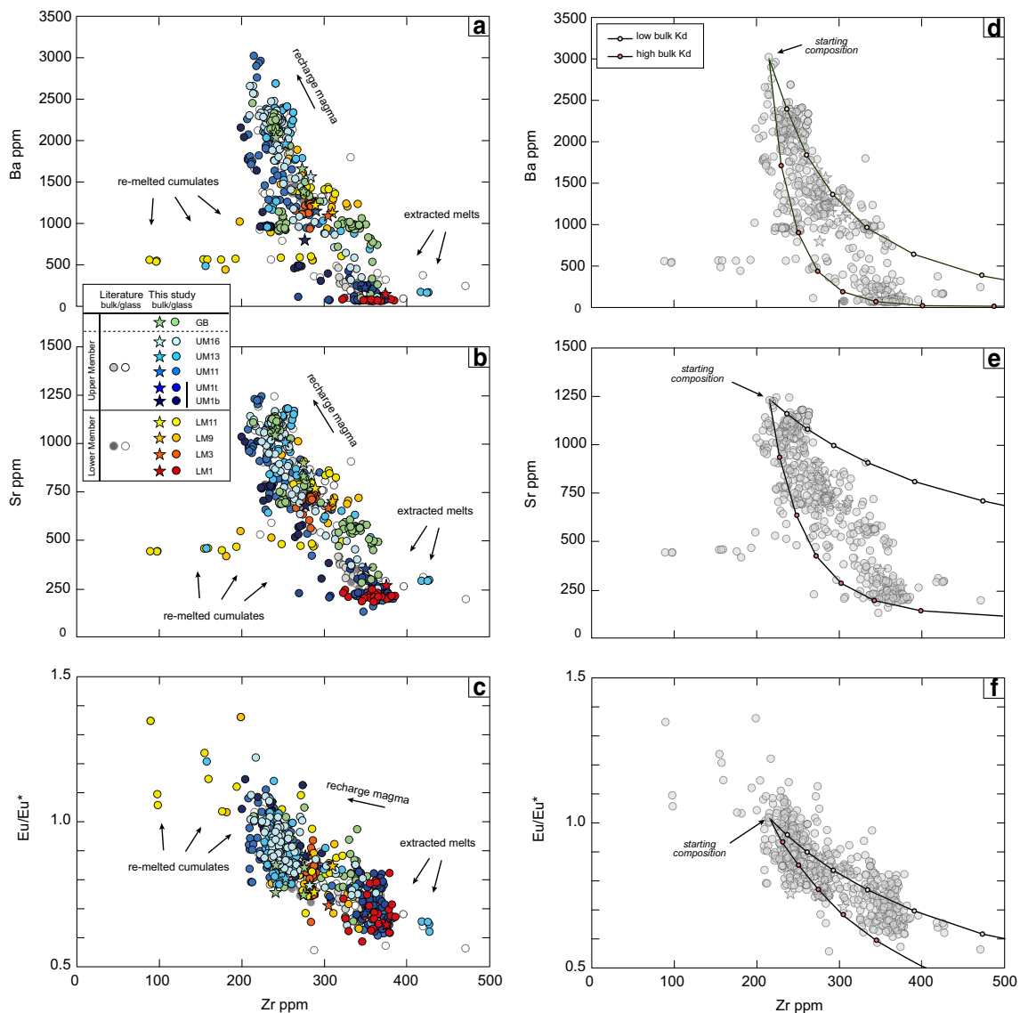
Fig. 4 Binary plots of and Zr (ppm) vs. Ba (ppm) (a), Sr (ppm) (b) and Eu/Eu^* [ =Eu_N/(Sm_N \times Gd_N)^{1/2} ; trace element concentrations normalized to values from McDonough and Sun, 1995] (c) of bulk-rocks (color-filled symbols) and matrix glasses (white-filled symbols) from the NYT. Grey symbols refer to data from the literature (Orsi et al. 1992, 1995; Scarpati et al. 1993; Wohletz et al. 1995;
