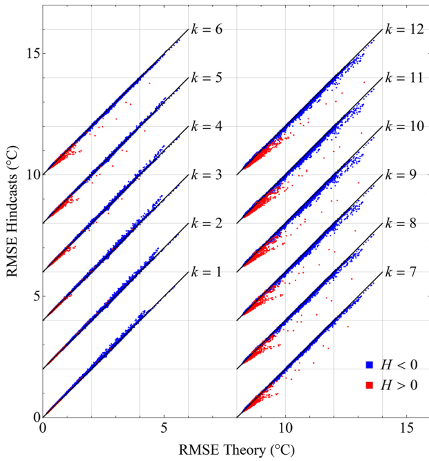
Fig. 6 Scatter plots for each horizon including the 10,512 grid points, showing the verification RMSE obtained from hindcasts vs. the expected theoretical RMSE_{nat}^{theory} predicted by Eq. (27). The graphs were displaced vertically by 2 °C (plus a horizontal displacement of 8 °C for k \geq 7 months) for visual clarity. The black line at 45° is a reference indicating perfect agreement between theory and verification. The blue points represent locations where H < 0 and the natural variability is modeled as an fGn process and the red points are for places where H > 0 and we use the fBm model
