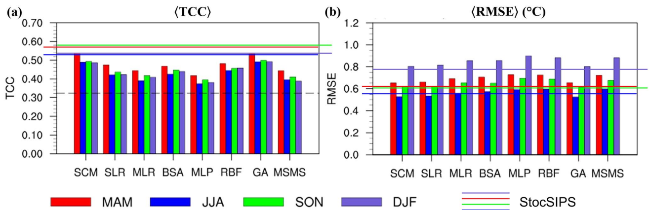
Fig. 17 Globally averaged TCC (a) and RMSE (b) (Eqs. (42) and (39), respectively) for MAM (red), JJA (blue), SON (green) and DJF (purple) for the period 1983–2009. The bars are for the MME combination methods in Kim et al. (2020), together with the mean of single model skills (MSMS). The scores for StocSIPS were included as
