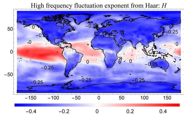
Fig. 2 Map of the fluctuation exponents obtained from the Haar fluctuation analysis (Lovejoy and Schertzer 2012a), in the high-frequency scaling regime between 2 months and 2 years
