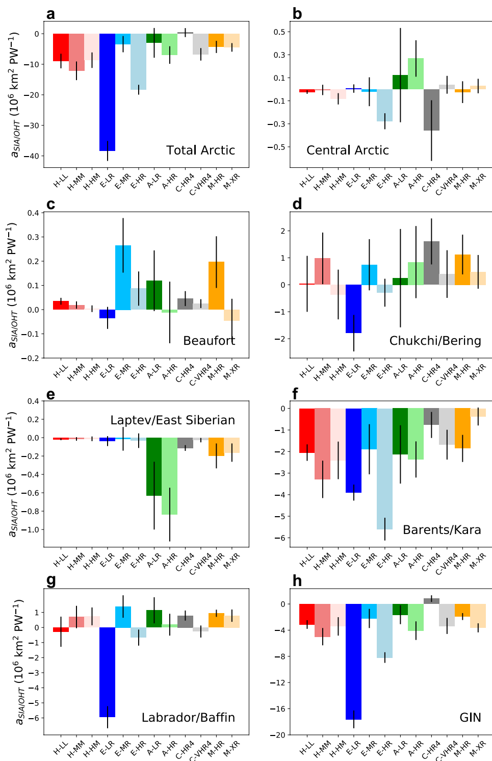
Fig. 14 Regression slopes ( a_{SIA/OHT} ) between detrended March Arctic sea-ice area and detrended annual mean Atlantic OHT at 70°N (computed over 1950–2014) for a the whole Arctic and b–h seven specific Arctic regions (GIN stands for Greenland–Iceland–Norwegian). The X axis shows the 12 model configurations used, with the first letter indicating the model (H: HadGEM3; E: ECMWF-IFS; A: AWI-CM; C: CMCC-CM2; M: MPI-ESM). The black line on top of each bar indicates the standard deviation of these slopes
