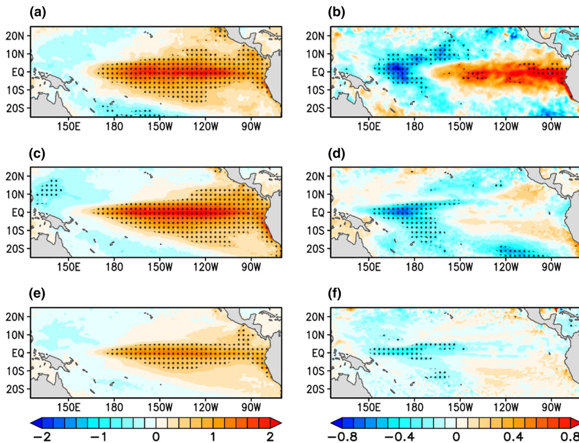
Fig. 4 Composite of December-January-February SSTA for symmetric (left-column) and asymmetric (right-column) component of ENSO for observed ( a , b ), HRCTL ( c , d ), and HRIE model ( e , f ) respectively. The symmetric component is defined by warm minus
