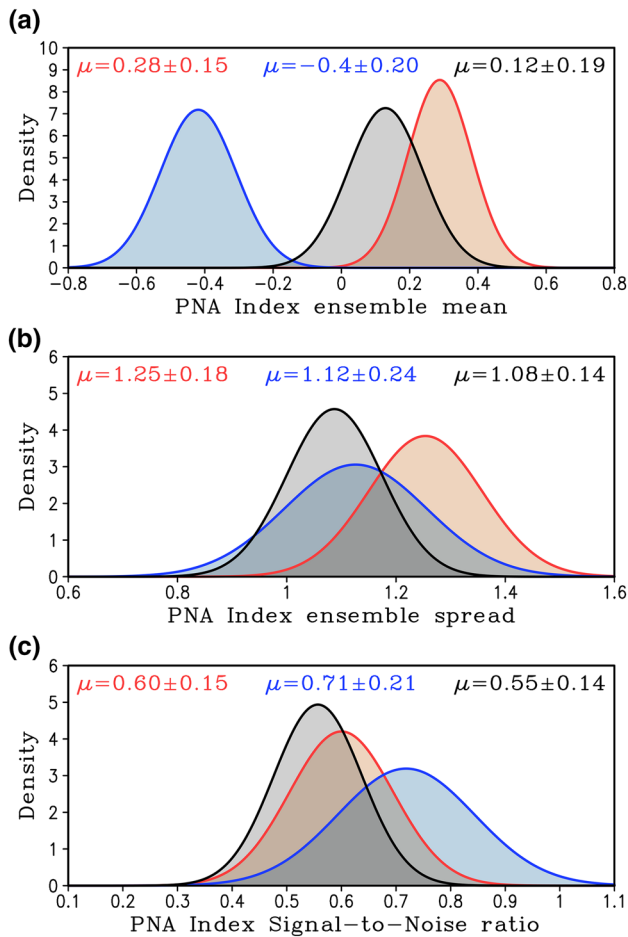
Fig. 15 Probability density function (PDF) of the PNA index conditioned by the state of Niño3.4 SSTA for El Niño (red), La Niña (blue), and neutral conditions (gray) in the HRIE experiment. a The ensemble mean PNA index, b the ensemble spread of the PNA index, and c the signal-to-noise ratio (SNR). The PDF were constructed by randomly selecting 6 out of 10 ensemble members from the HRIE experiment and computing the ensemble mean, spread, and SNR for each realization, this was repeated 1000 times. The mean plus the 95th percentile is shown at the top of each panel
