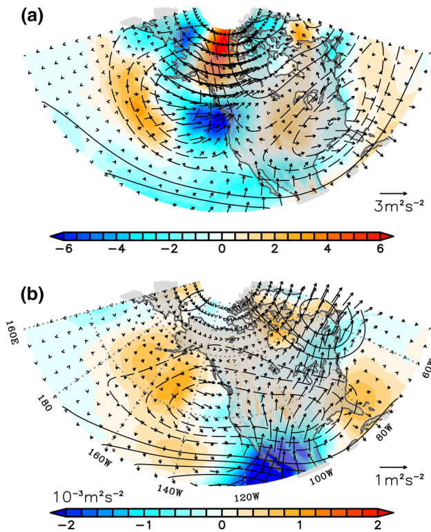
Fig. 11 Composite of December–January–February (DJF) seasonal mean 200 hPa anomalous streamfunction ( 10^6 \text{ s}^{-1} , contour), horizontal (vector) and vertical (shaded) stationary Rossby wave flux during El Niño events for HRCTL (a) and HRIE (b). Composite is defined based on the top 10 strongest El Niño events
