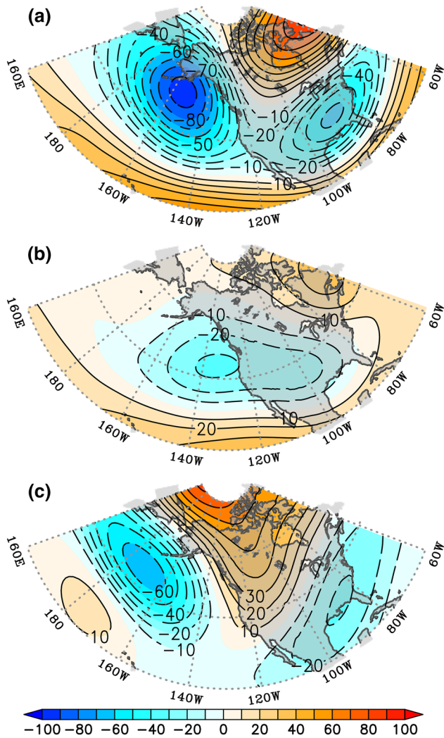
Fig. 8 Composite of 200 hPa geopotential height anomaly during DJF for warm ENSO events for HRCTL model (a) and HRIE model (b). Also showing the spatial structure of EOF 1 of internal atmospheric dynamics 200 hPa geopotential height for HRIE model (c). Contour interval is 10 m for all panels
