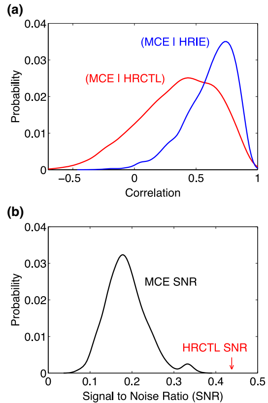
Fig. 9 Probability density function (PDF) for the spatial correlation between MCE and HRCTL composite (red) and the spatial correlation of MCE and HRIE composite (blue) of midlatitude 200 hPa geopotential height anomaly during El Niño events (a). b PDF of signal-to-noise ratio (SNR) of MCE composite (black) compared to HRCTL SNR (red arrow). The MCE are built by 5000 realizations using a Monte Carlo sampling technique
