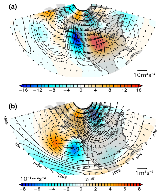
Fig. 3 Conditional composite of 200 hPa anomalous streamfunction (contour), horizontal (vector) and vertical (shaded) stationary Rossby wave flux of December–January–February (DJF) seasonal mean during a positive PNA and neutral ENSO, and b positive ENSO events and neutral PNA. Streamfunction contour interval is 3 \times 10^6 \text{ s}^{-1} for (a) and 10^6 \text{ s}^{-1} for (b)
