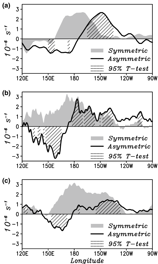
Fig. 13 Composite of observed (a), HRCTL (b), and HRIE (c) symmetric (i.e., El Niño minus La Niña divided by 2, shaded grey) and asymmetric (El Niño plus La Niña, black line) components of 200 hPa anomalous divergence meridionally averaged (5S–5N) across the Pacific Ocean. Dotted shade indicates where the asymmetry is distinct from zero at 95% confidence level from a student-T test. The analysis of HRIE model is performed on the ensemble mean from the 10 atmospheres realization
