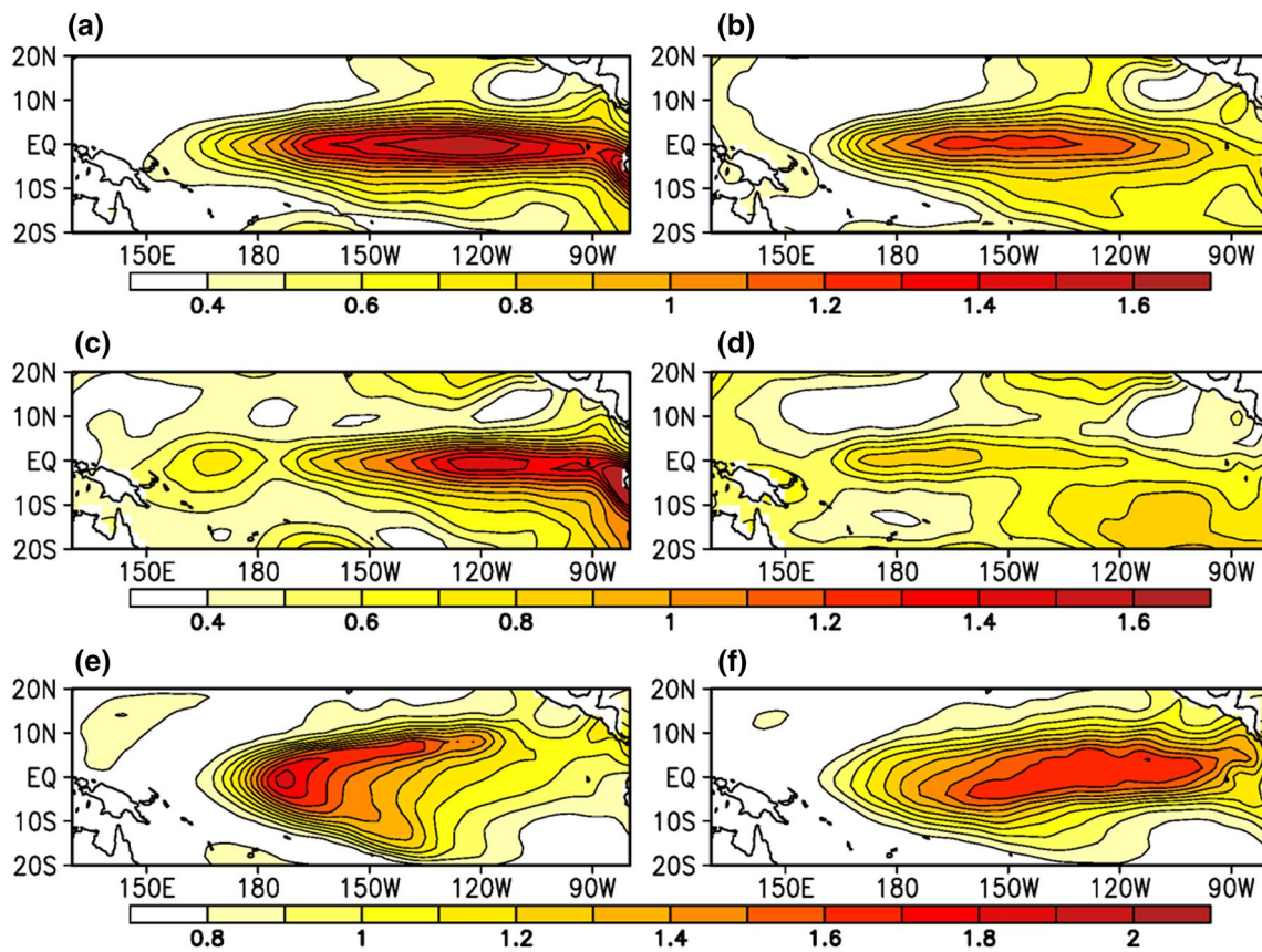
Fig. 16 a Ensemble mean (i.e., signal), c ensemble spread (i.e., noise), and e signal-to-noise ratio of observed SST anomaly during El Niño events for the period of 1950–2017. b , d , and f are similar to a , c , e but for La Niña SST anomalies. The ensemble mean is taken as
