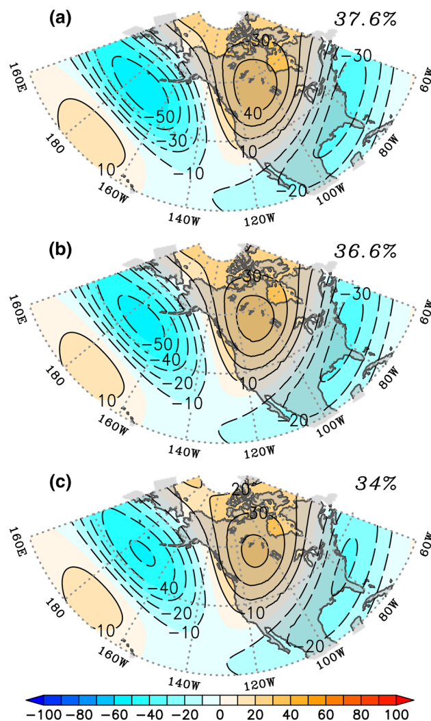
Fig. 10 The spatial structure of EOF 1 of internal atmospheric dynamics of 200 hPa geopotential height for HRIE model for; a El Niño, b La Niña, and c Neutral boreal winters. Contour interval is 10 m for all panels. The percentage values indicate the variance explained by this EOF 1
