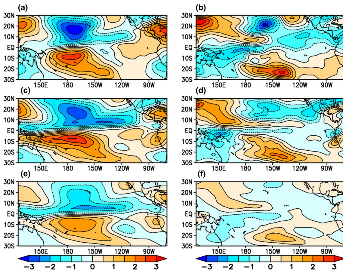
Fig. 5 Same as in Fig. 4 but for the Rossby wave source. Contour interval is 0.5 \times 10^{-11} \text{ s}^{-2} . Anticyclonic (cyclonic) wave source is negative (positive) in the Northern Hemisphere and the opposite in the Southern Hemisphere
