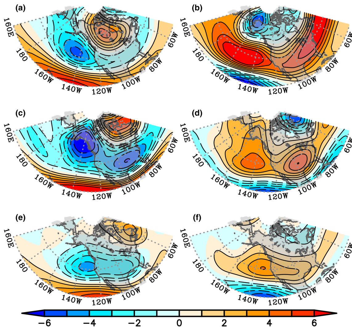
Fig. 14 Composite of 200 hPa streamfunction anomaly ( 10^6 \text{ s}^{-1} ) for boreal winters (DJF) during El Niño events: observed (a), HRCTL (c), and HRIE (e). Similarly, for La Niña events: observed (b), HRCTL (d), and HRIE (f)
