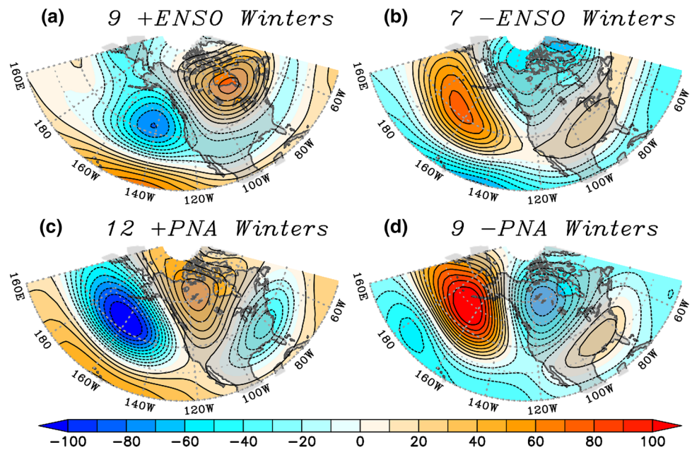
Fig. 1 Composite of 200 hPa geopotential height anomaly during DJF for warm ENSO events (a), cold ENSO events (b), warm PNA winters (c), and cold PNA winters (d). Contour interval is 10 m. The number in each sub-title corresponds to the number of events in the composite
