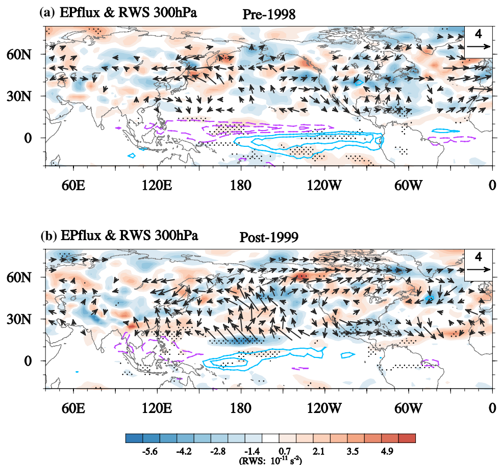
Fig. 5 Regression maps of the 300-hPa Rossby wave source (RWS) (shading; unit: \text{s}^{-2} ), horizontal Plumb flux (vector; unit: \text{m}^2 \text{s}^{-2} ) and vertically integrated diabatic heating anomalies (contour; unit: \text{W m}^{-2} ) onto the a pre-1998 PC1 and b post-1999 PC1. The contour interval for diabatic heating is 4.0 \text{ W m}^{-2} . The stippling indicates significance at the 95% confidence level
