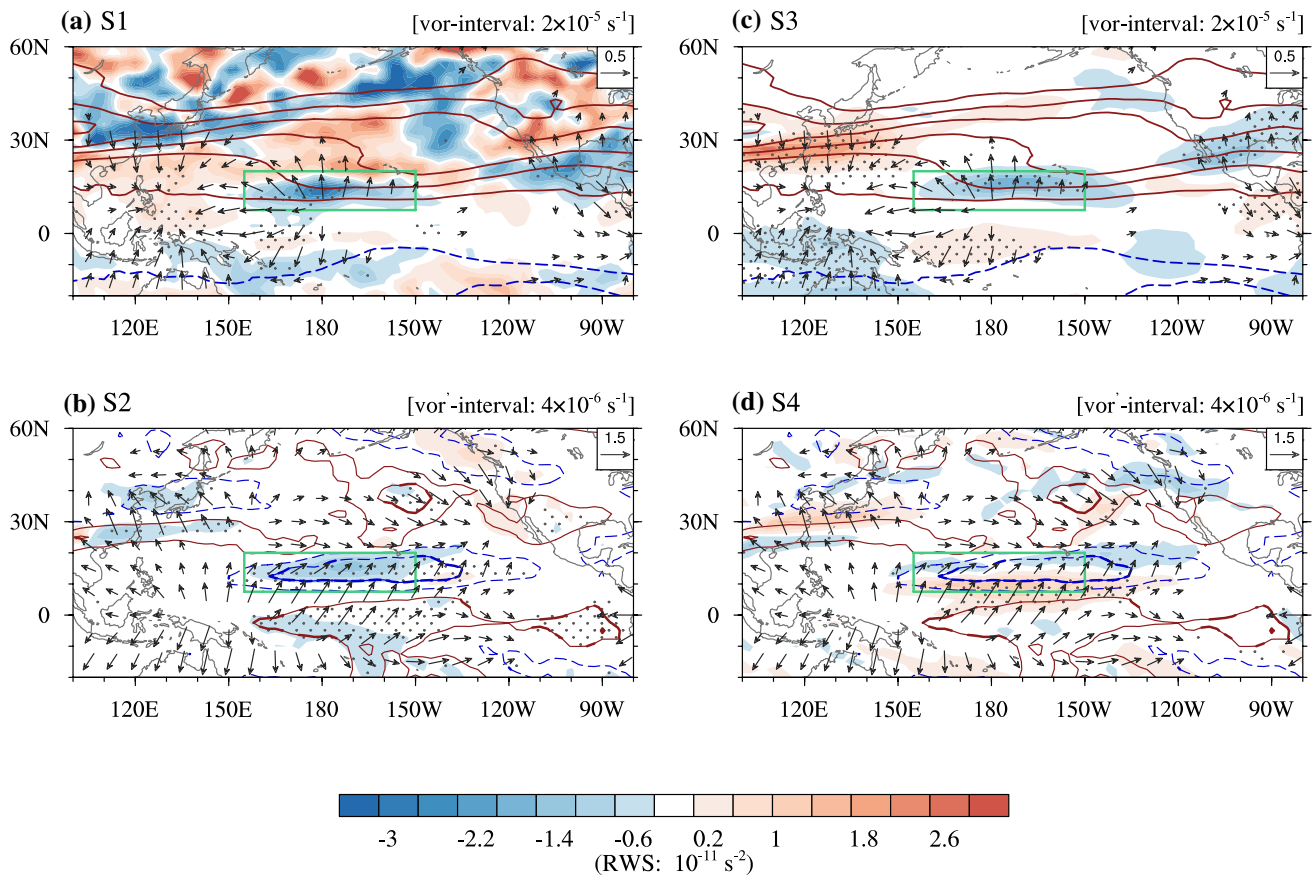
Fig. 8 Same as Fig. 7, but onto the post-1999 PC1. The mean absolute vorticity and divergence wind are averaged during 1999–2016. The boxes denote the area ( 7.5^{\circ}\text{N} – 20^{\circ}\text{N} ; 155^{\circ}\text{E} – 150^{\circ}\text{W} )
