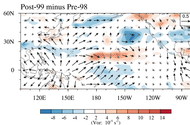
Fig. 11 The differences of mean absolute vorticity (shaded; unit: \text{s}^{-1} ) and divergence wind (vector; unit: \text{m s}^{-1} ) between the pre-1998 and post-1999 periods (post-1999 minus pre-1998). The stippling and thick vectors indicate differences at or above the 95% confidence level
