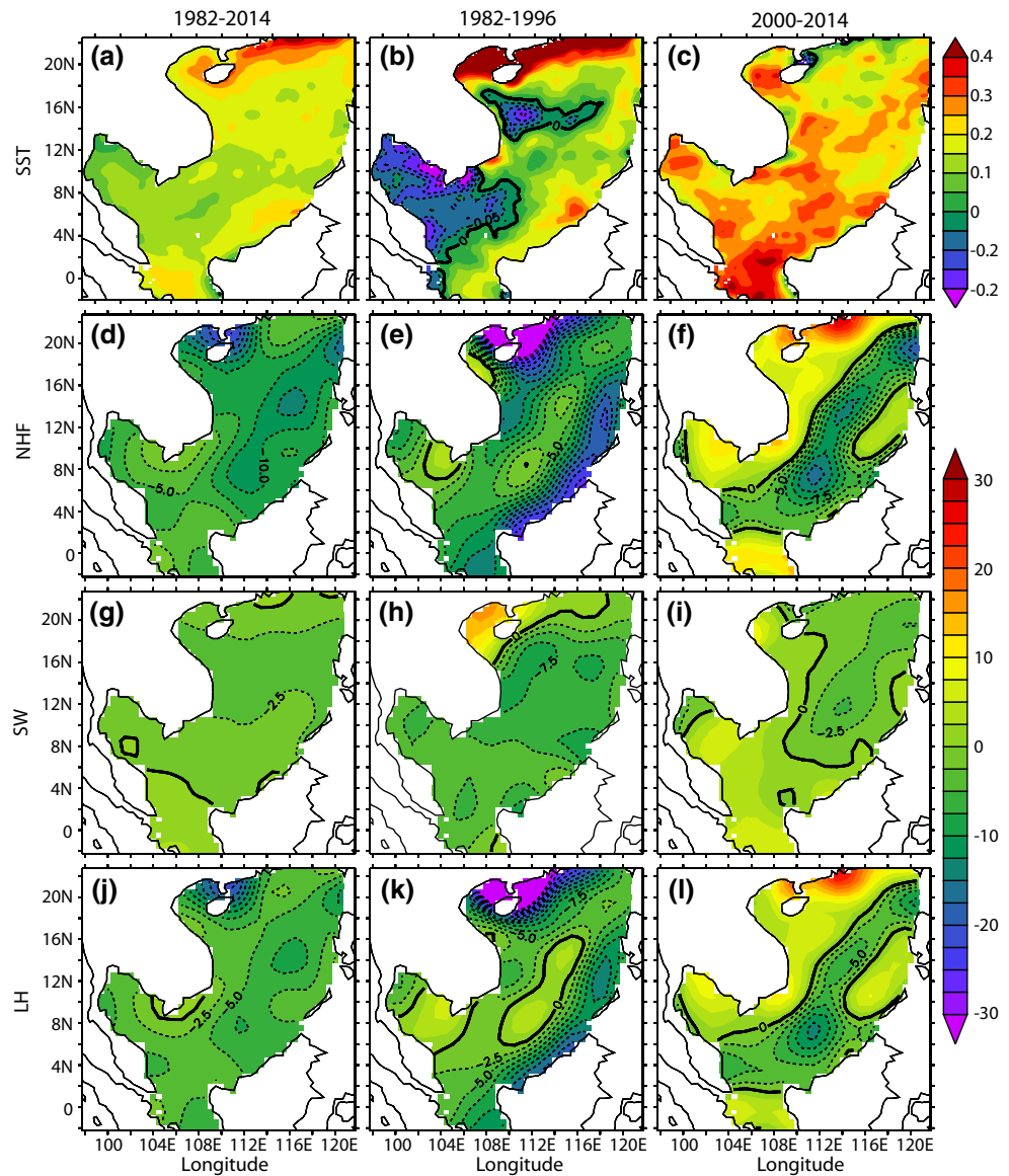
Fig. 5 The linear trends of SST in °C per decade (a–c), net surface heat flux in \text{w m}^{-2} per decade (d–f), short wave flux in \text{w m}^{-2} per decade (g–i) and latent heat flux \text{w m}^{-2} per decade (j–l) over the SCS. The linear trends during 1982–2014, 1982–1996 and 2000–2014 are shown in the left, middle and right panels respectively. The top color bar represents the SST trend while the heat flux trends are indicated by the bottom color bar. The contours represent negative values
