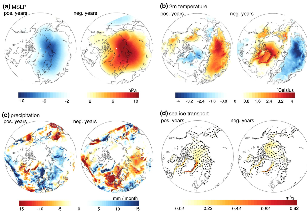
Fig. 6 EOF 1 composites: Difference between DJF mean of the positive years ( left ) and the negative years ( right ) and the overall mean of DJF of a MSLP in hPa, b 2 m temperature in °C, and c precipitation in mm month -1 . The grey contour line indicates the region where
