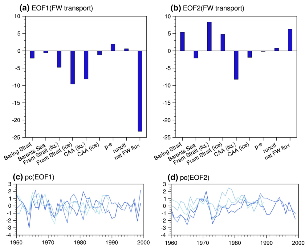
Fig. 3 a Leading and b second leading empirical orthogonal function (in mSv) of the FW transports, including the net FW flux, in the Arctic. The explained variance is about 33 and 18 %, respectively. The corresponding normalized PCs, obtained by projecting the different ensemble members onto the EOFs, are presented in c and d
