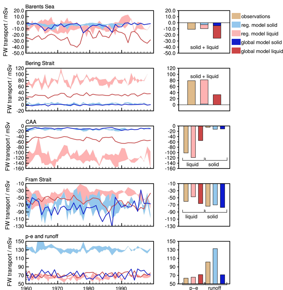
Fig. 2 Left column Time evolution (yearly values) of the FW components from the regional model and the global model. The ensemble spread is defined by minimum and maximum values of the ensemble members, for liquid and for solid FW transport (in light red and light blue ). Liquid and solid FW transport of the global model is given in red and blue , respectively. For the last panel, p-e is given in red and runoff in blue . Right column Mean value of the time series of the regional model (ensemble mean) and the global model and from observations and reanalysis data from Serreze et al. (2006)
