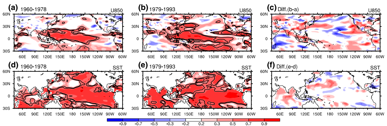
Fig. 5 Temporal correlation coefficients (TCC) of JJA-mean 850-hPa zonal wind (upper) and SST anomalies (lower) between the observations and MME predictions during 1960–1978 (left), 1979–1993
