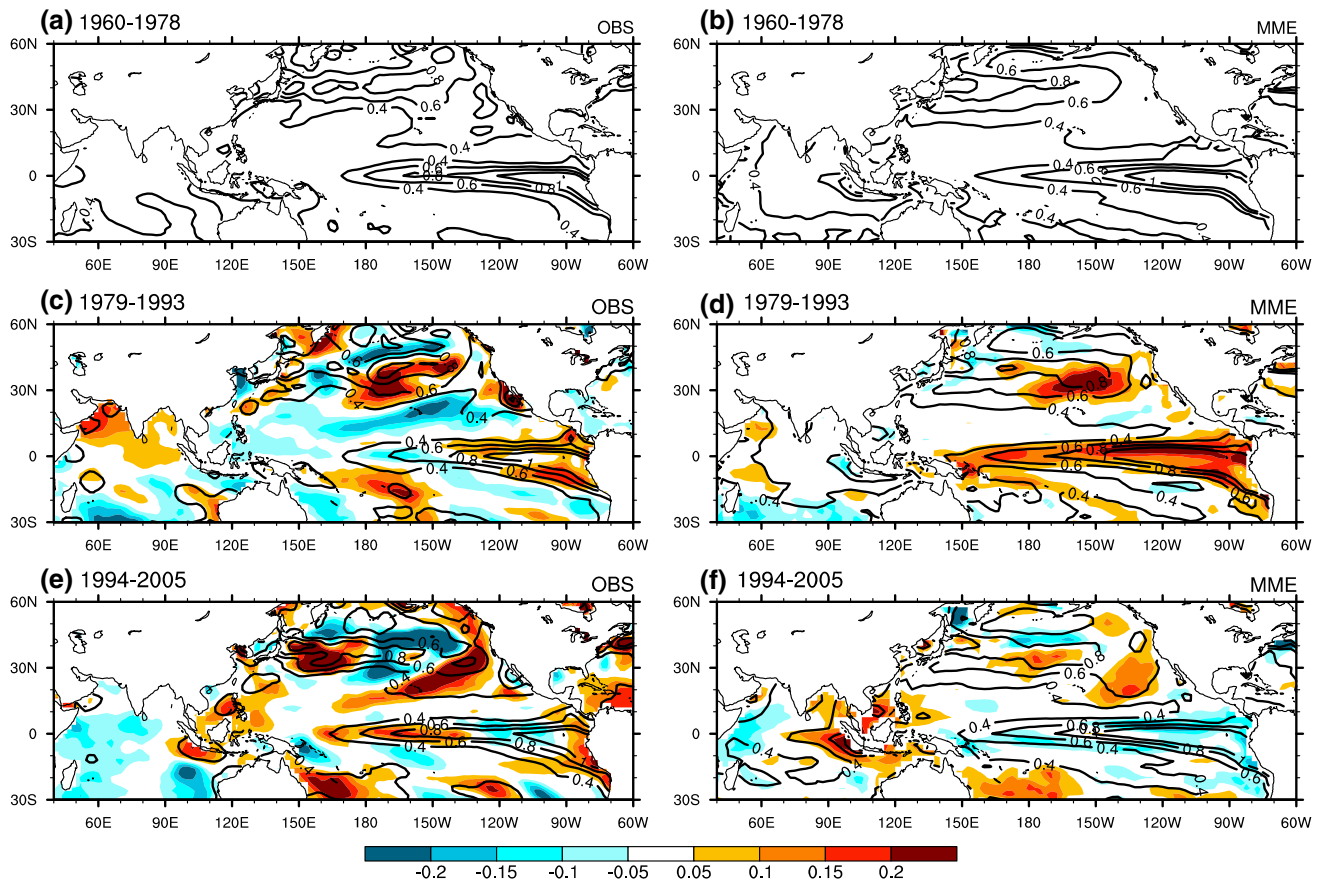
Fig. 2 Similar to Fig. 1, but for the interannual variability of the JJA-mean SST
