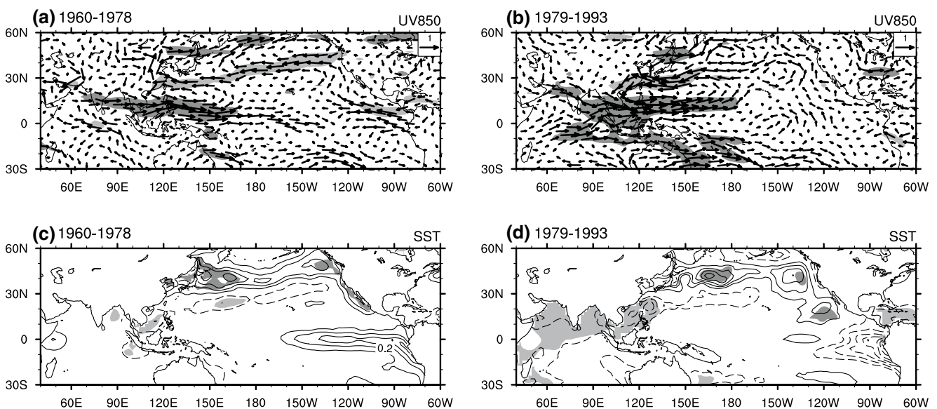
Fig. 7 Regression of the 850-hPa winds ( upper ) and SST ( lower ) anomalies onto the normalized WNPMI in observations during 1960–1978 ( left ) and 1979–1993 ( right ). The shading indicates the regions
