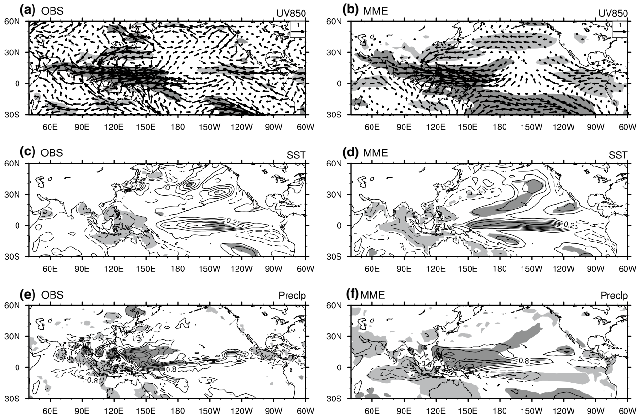
Fig. 9 Regression of the 850-hPa zonal wind ( upper ), SST ( middle ) and precipitation ( lower ) anomalies onto the normalized WNPMI in observations ( left ) and the ENSEMBLES MME prediction ( right )
