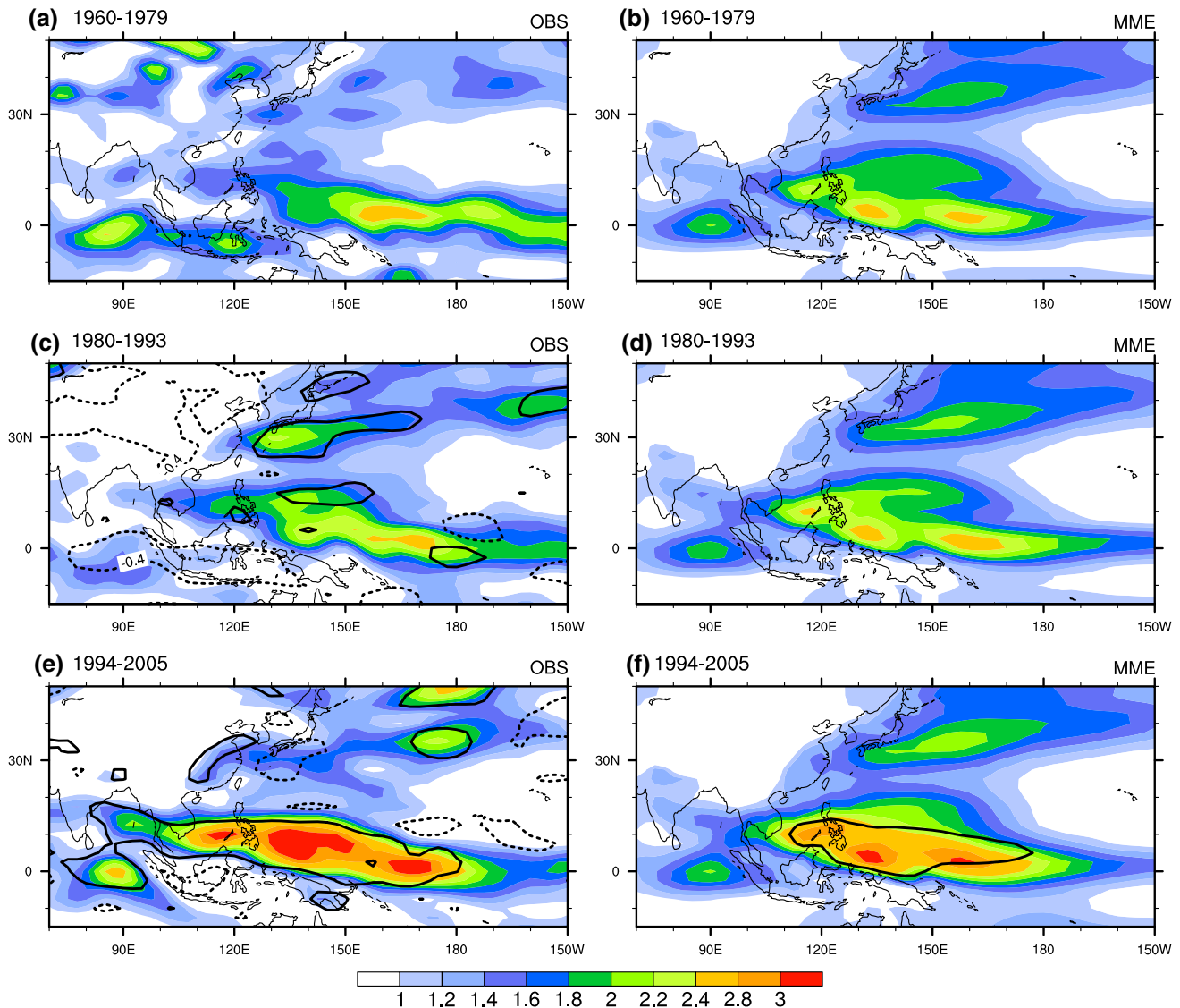
Fig. 3 Interannual variability of 850-hPa zonal wind for observations ( left ) and the ENSEMBLES MME prediction ( right ). Unit: \text{m s}^{-1} . The contours represent where differences of SD to previous period are larger (smaller) than 0.4 ( -0.4 ) \text{m s}^{-1}
