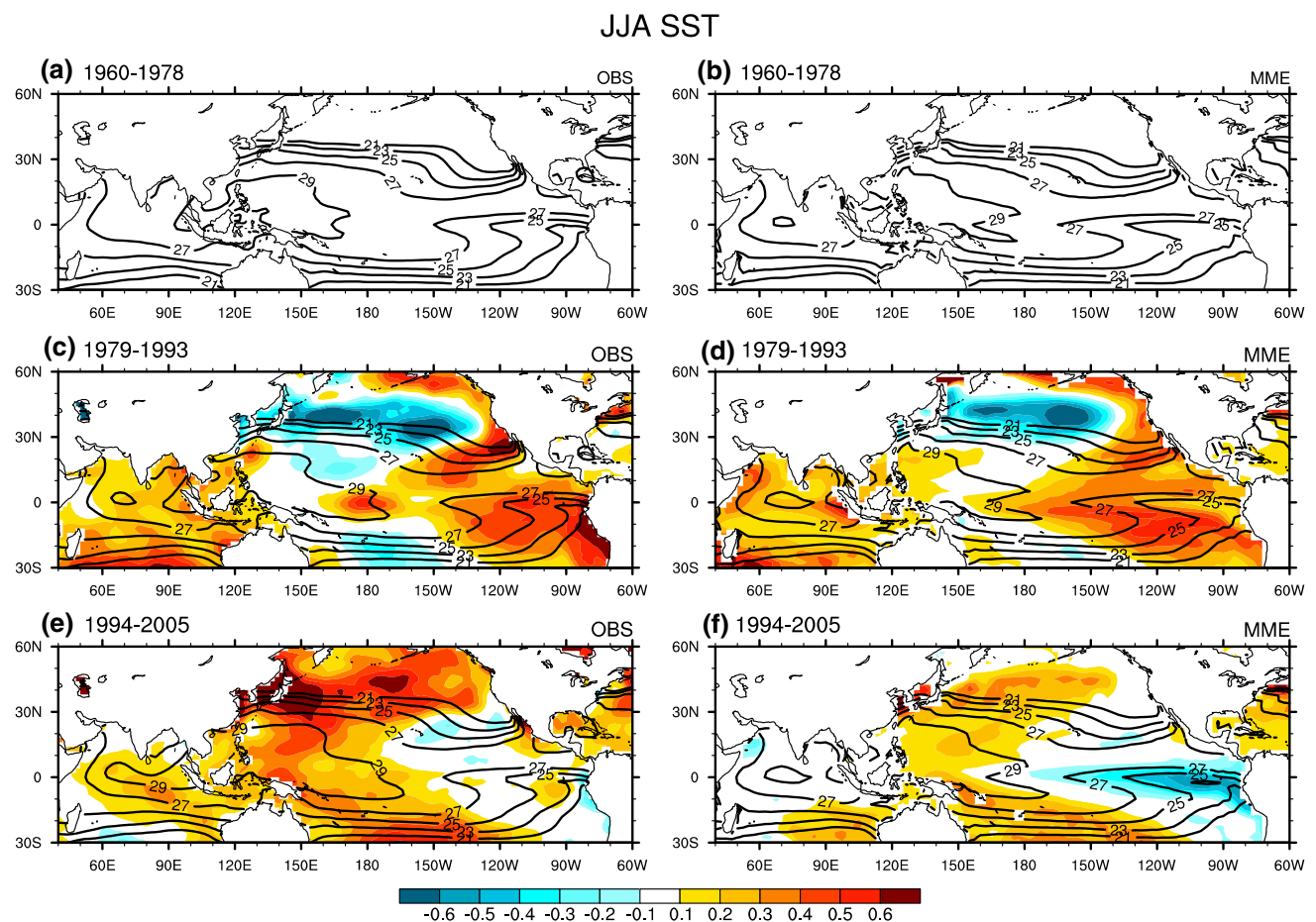
Fig. 1 Climatology of JJA-mean SST for observations (left) and the ENSEMBLES MME prediction (right) during 1960–1978 (upper), 1979–1993 (middle) and 1994–2005 (lower). Unit: °C. The shading represents differences of SST to the previous period
