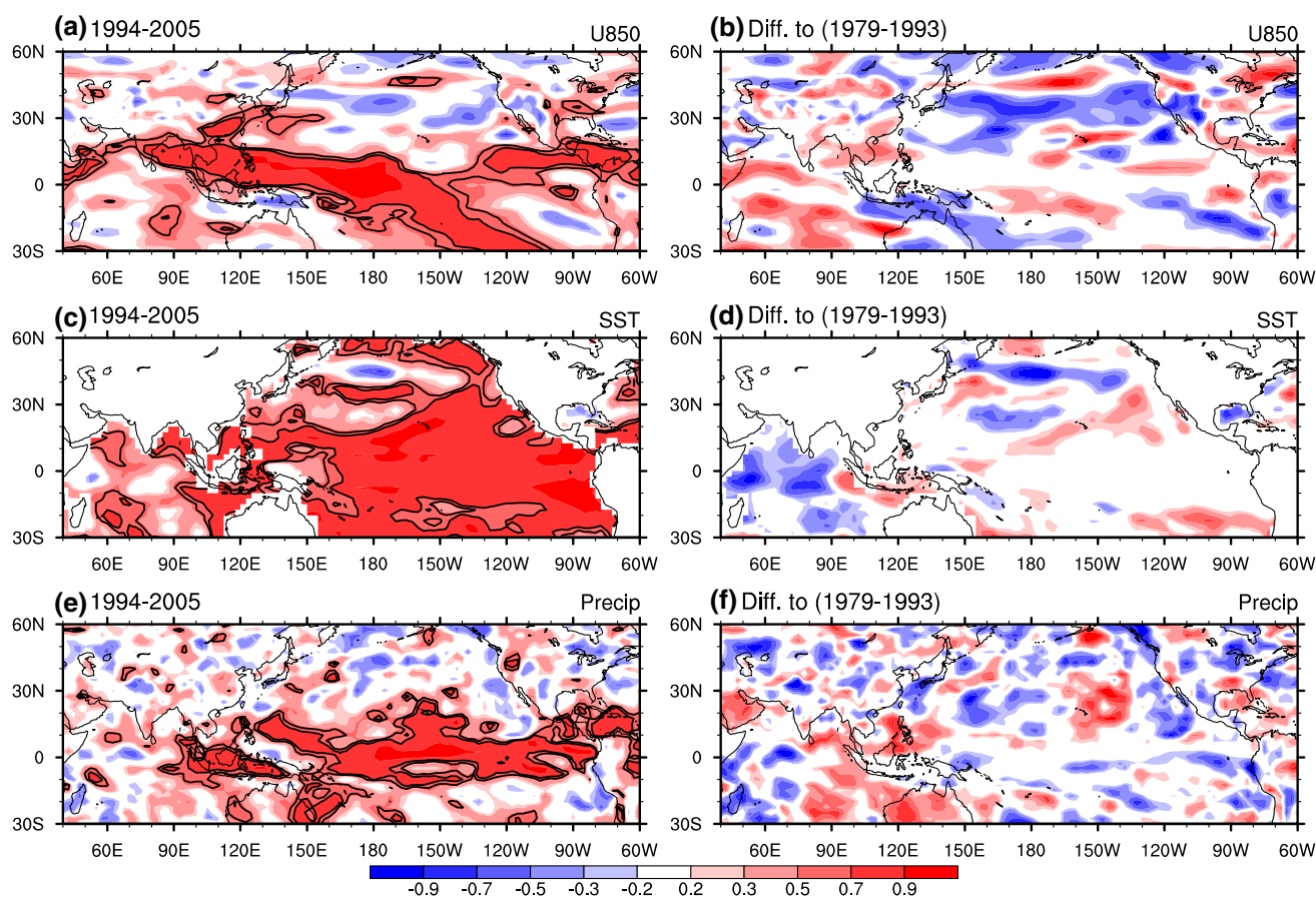
Fig. 6 Same as Fig. 5, but for the TCC of JJA-mean 850-hPa zonal wind ( upper ), SST ( middle ) and precipitation ( lower ) anomalies during 1994–2005 ( left ) and the differences ( right ) to that during 1979–1993
