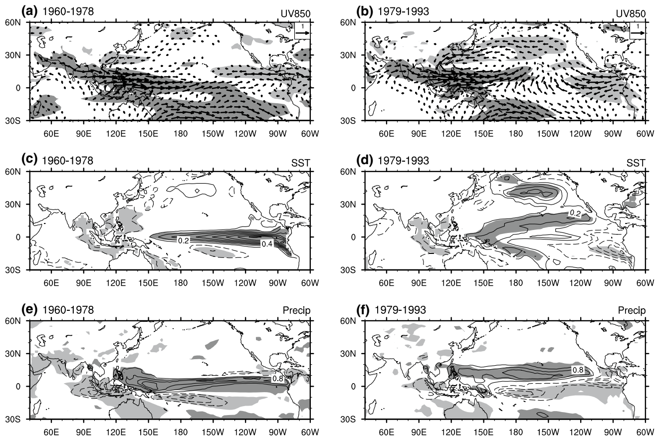
Fig. 8 Same as Fig. 7, but for the 850-hPa zonal wind ( upper ), SST ( middle ) and precipitation ( lower ) anomalies in the ENSEMBLES MME prediction. Interval of the precipitation anomaly is 0.4 \text{ mm day}^{-1}
