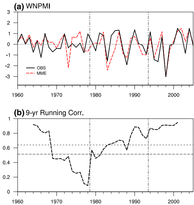
Fig. 4 a Time series of the normalized WNP summer monsoon index (WNPMI) for observations ( solid black line ), the MME predictions ( dashed red line ) and b the 9-year running correlation of the WNPMI between the observations and MME predictions. The dashed lines in b represent statistical significance of the correlation coefficients at 95 and 99 % confidence levels, respectively
