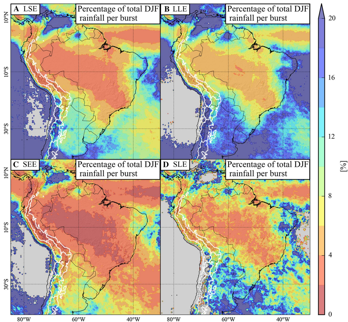
Fig. 6 Average percentage of total DJF rainfall contributed by each single burst of consecutive events of type local and short ( a LSE), local and long-lasting ( b LLE), spatially extensive ( c SEE), and spatially extensive long-lasting ( d SLE)
